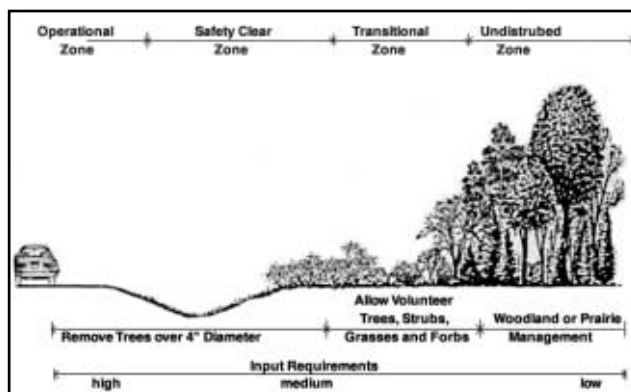
Figure 4-2. Roadway Zones
