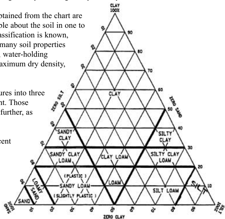
Figure B-1. Soil Classification
