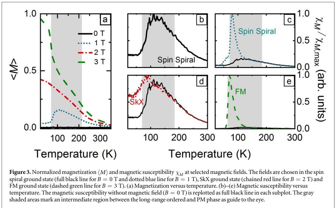
Figure 2. Energy \langle E \rangle and heat capacity C at selected magnetic fields. (a) Energy \langle E \rangle versus temperature. The four energy curves for the magnetic fields 0–3 T lie on top of each other in panel (a). (b) Heat capacity versus temperature. The dotted line defines the critical temperature T_c between the long or short range ordered phase to the disordered phase.
