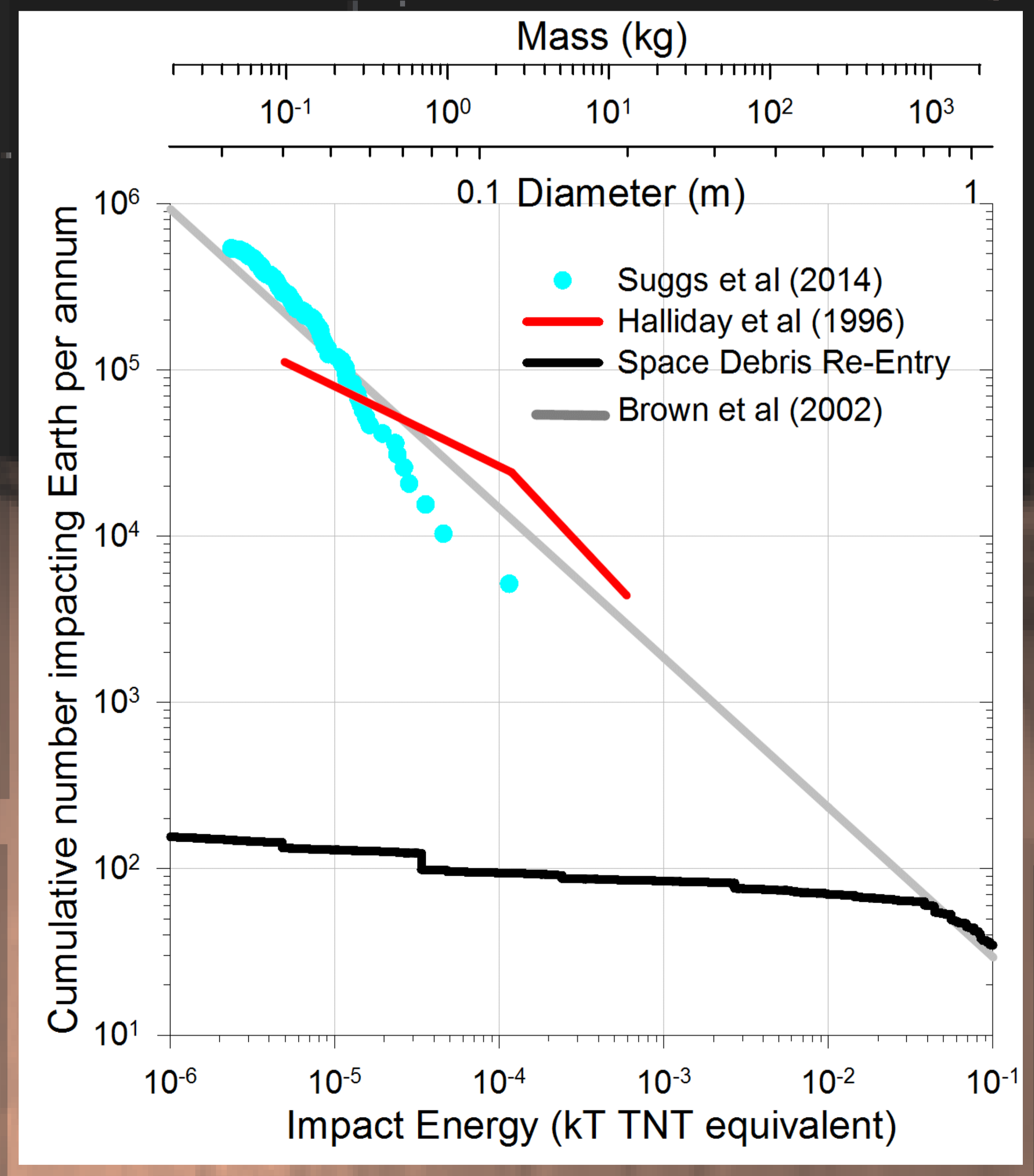
Figure 4: Meteoroid flux at the top of the atmosphere based on photographic network measurements of the Meteorite and Observation and Recovery Project [MORP] (Halliday et al (1996)), lunar impact flashes (Suggs et al, 2014) and global bolide flux estimates (power law fit to data shown) for impactors with energies larger than 0.1 kJ (Brown et al 2002). Also shown for comparison are the cumulative annual number of space debris re-entries, where the mass of the debris at the top of the atmosphere is shown.
