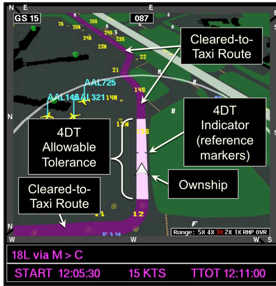
Fig. 2. Airport Moving Map (AMM) in the defined -tolerance display format with 4DT indicator (black reference lines in front of the ownship) and +/-405 ft allowable tolerance (light pink band).
