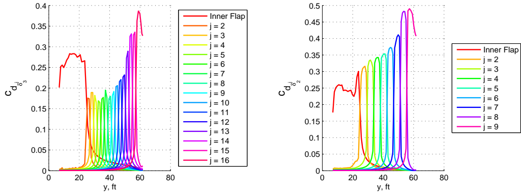
Figure 56. Stiff Wing Low-Speed Take-Off Sectional Drag Spanwise Derivatives to VCCTEF, c_{d_{\delta_n}}(y) (VCCTEF configuration #1, left, VCCTEF configuration #2, right)
