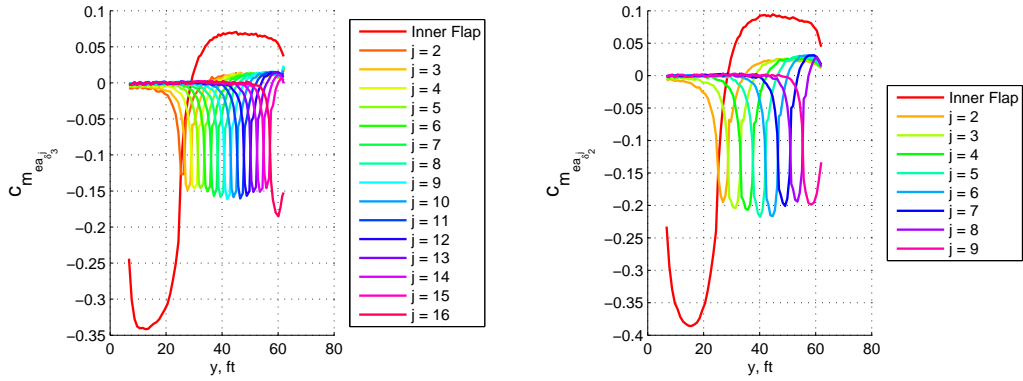
Figure 16. Rigid Wing Cruise Sectional Pitching Moment (about Elastic Axis) Spanwise Derivatives to VCCTEF, C_{m_{ea\delta_n}}(y) (VCCTEF configuration #1, left, VCCTEF configuration #2, right)
