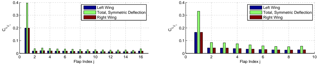
Figure 59. Stiff Wing Low-Speed Take-Off Total Aircraft Lift Derivatives to VCCTEF, C_{L_{\delta_n}} (VCCTEF configuration #1, left, VCCTEF configuration #2, right)
