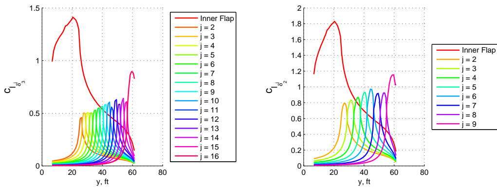
Figure 33. Flexible Wing Cruise Sectional Lift Spanwise Derivatives to VCCTEF, C_{l_{\delta_n}}(y) (VCCTEF configuration #1, left, VCCTEF configuration #2, right)
