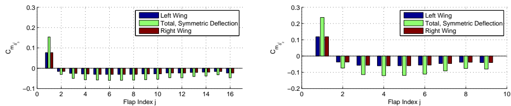
Figure 41. Flexible Wing Cruise Total Aircraft Pitching Moment Derivatives to VCCTEF, C_{m_{\delta_n}} (VCCTEF configuration #1, left, VCCTEF configuration #2, right)
