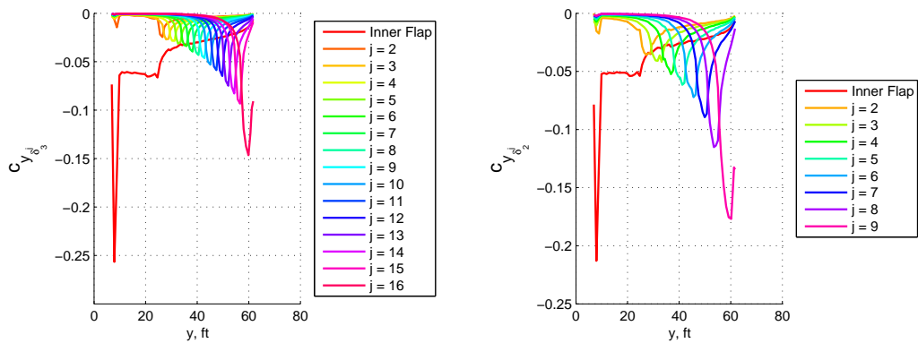
Figure 57. Stiff Wing Low-Speed Take-Off Sectional Side Force Spanwise Derivatives to VCCTEF, c_{y_{\delta_n}}(y) (VCCTEF configuration #1, left, VCCTEF configuration #2, right)
