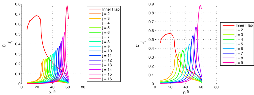
Figure 65. Flexible Wing Low-Speed Take-Off Sectional Lift Spanwise Derivatives to VCCTEF, c_{l_{\delta_j}}(y) (VCCTEF configuration #1, left, VCCTEF configuration #2, right)
