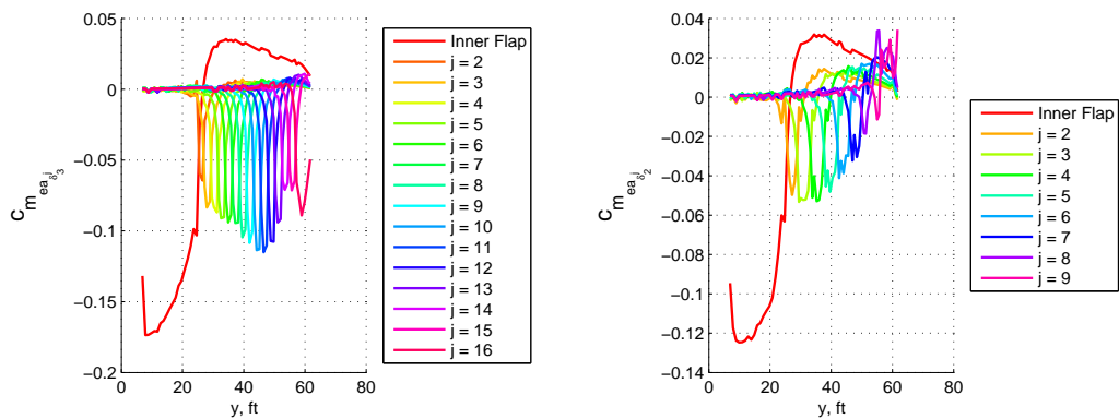
Figure 58. Stiff Wing Low-Speed Take-Off Sectional Pitching Moment (about Elastic Axis) Spanwise Derivatives to VCCTEF, c_{m_{\text{ea}_{\delta_n}}}(y) (VCCTEF configuration #1, left, VCCTEF configuration #2, right)
