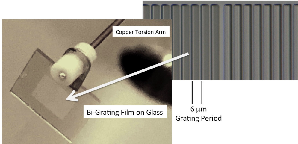
Photoresist bi-grating on glass, mounted in the RIT radiation pressure test-bed. Micro-fabrication by Rajesh Menon, U. Utah. Grating period: 6 \mu\text{m} .
