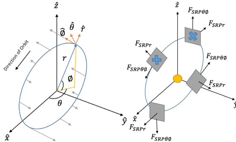
Left: Sun-centered spherical coordinate system with x,y ecliptic plane, azimuth \theta , polar angle above the ecliptic \phi , and radius r . Arrows represent radiation pressure force vectors. Right: Attitude of a diffraction sail with respective force components.
