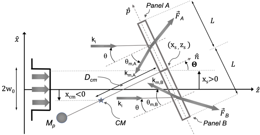
Fundamental elements of a diffractive bi-grating beam rider (patent pending).
