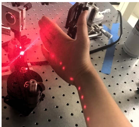
Left: Multiple diffraction orders of a low power HeNe laser beam from the U. Utah diffraction grating. Right: at t > 600 \text{ s} a 1.2W diode laser ( \lambda = 808 \text{ nm} ) provided significant radiation pressure, changing free oscillations into a forced oscillation state.
