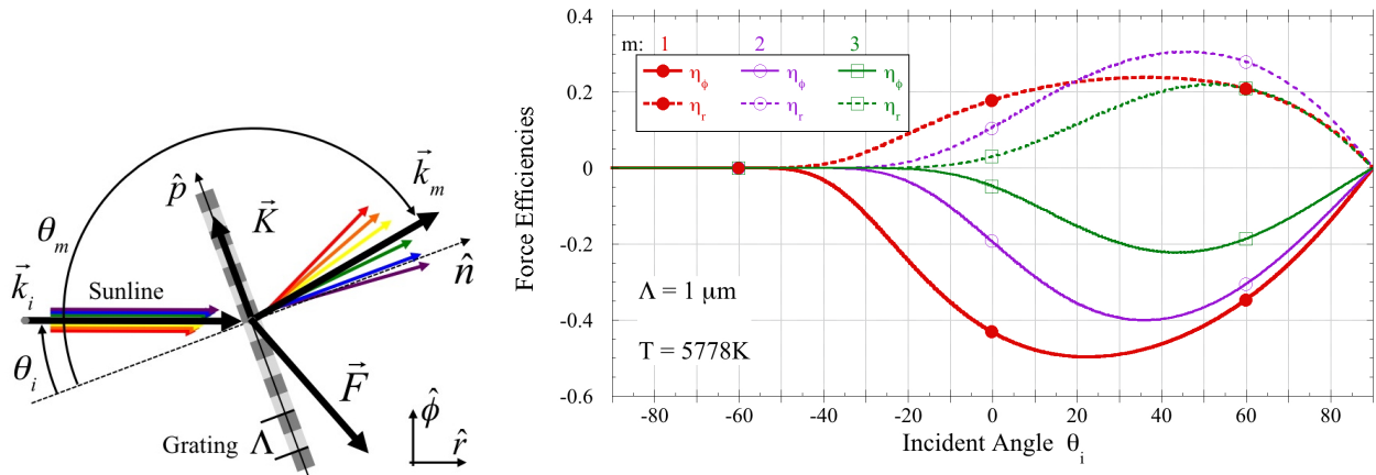
Left: Broadband sunlight is diffracted at different angles. Right: Components of force efficiency along the sun line \eta_r , and at right angle \eta_\phi for different diffraction orders m , calculated for a grating period \Lambda = 1 \mu\text{m} and the solar black body spectrum at temperature T = 5778 \text{ K} .
