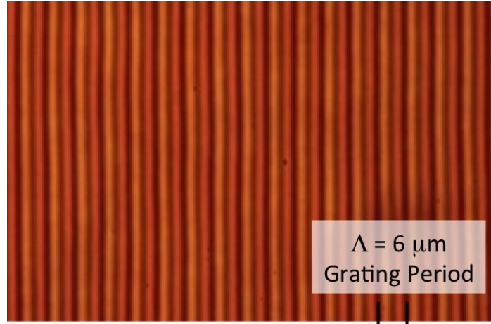
Magnified section of the BEAMCo diffractive film with grating period L = 6\mu\text{m} .
