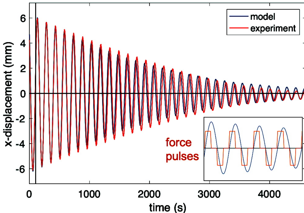
Radiation pressure “cooling” of an excited torsion oscillator. Inset shows laser pulses synchronized with the oscillation phase.
