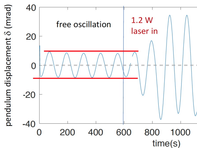
Left: Multiple diffraction orders of a low power HeNe laser beam from the U. Utah diffraction grating. Right: at t > 600 \text{ s} a 1.2W diode laser ( \lambda = 808 \text{ nm} ) provided significant radiation pressure, changing free oscillations into a forced oscillation state.
