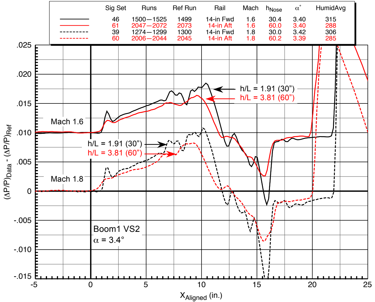
Figure 27. Effects of Boom1 VS2 model height, X sweeps 9x7 Parametric Test, P_T = 2297 psf
