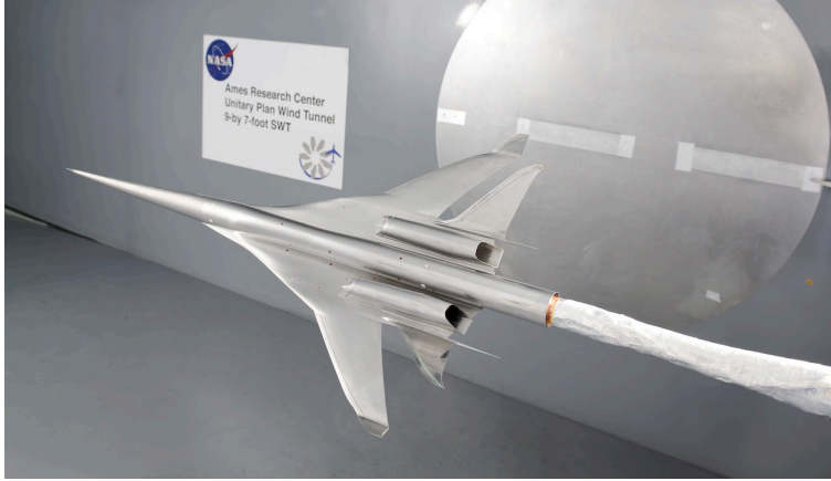
Figure 6. Rear view of Performance model in Ames 9x7 tunnel
