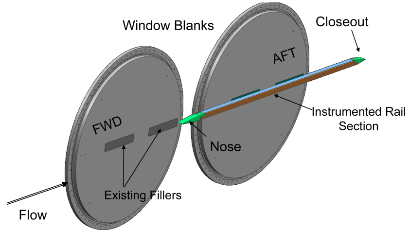
Figure 16. CAD view of 2” rail mounted on aft window blank of 9x7 wind tunnel
