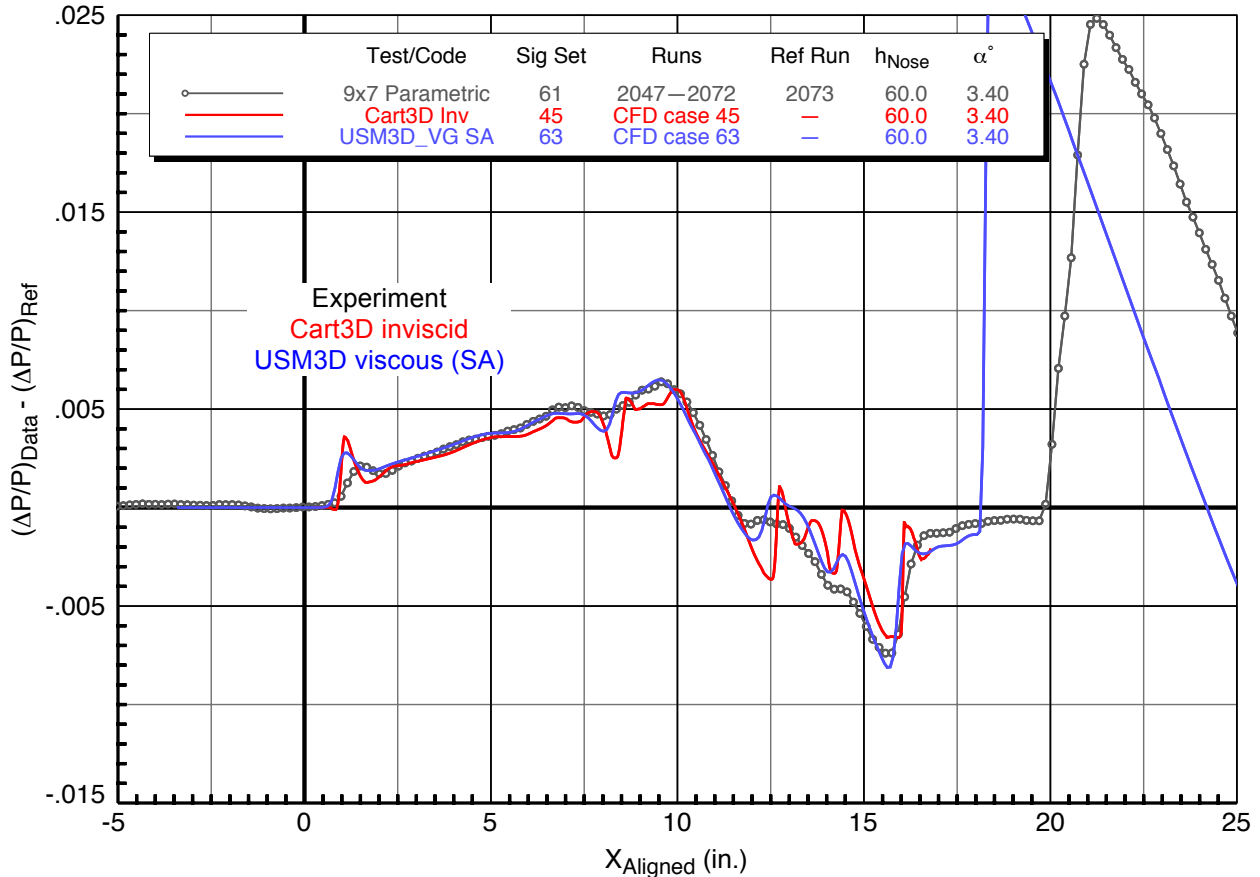
Figure 41. Experiment/CFD comparisons for Boom1 VS2 Model 9x7 Parametric Test, 14-in aft rail, Mach = 1.60, P_T = 2299 psf, HumidAvg = 288 ppm
