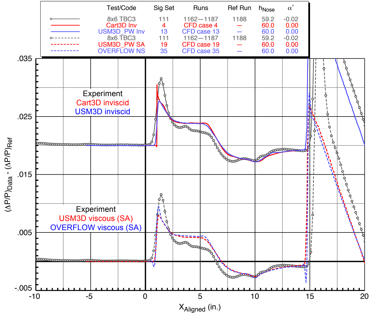
Figure 37. Experiment/CFD comparisons for AS2 Model 8x6 TBC3 Test, 2-in rail, M = 1.56 (WT), 1.60 (CFD), P_T = 2939 psf, HumidAvg = 66 ppm
