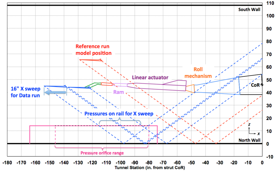
Figure 20. Layout of reference and data runs in 9x7 wind tunnel (view from floor of tunnel looking up)
