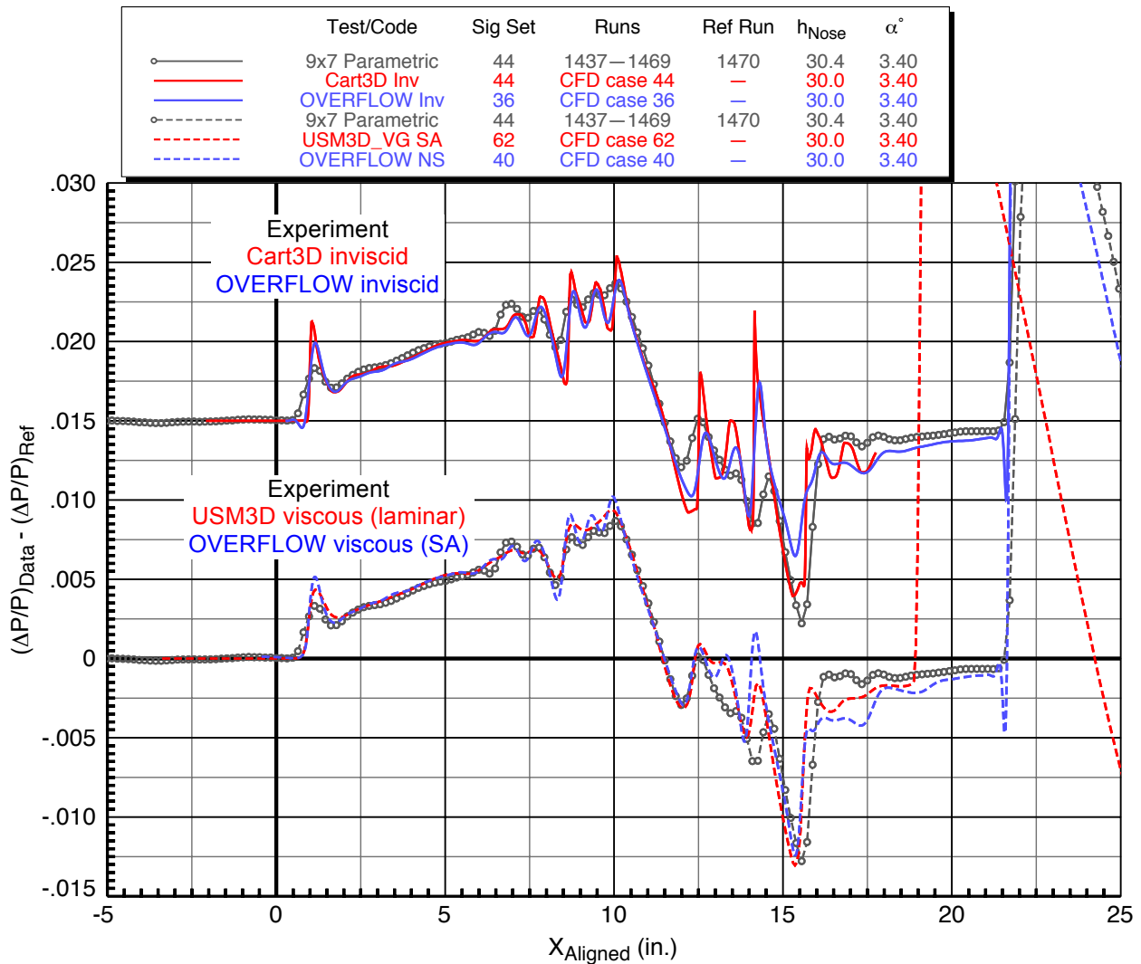
Figure 40. Experiment/CFD comparisons for Boom1 VS2 Model 9x7 Parametric Test, 14-in fwd rail, Mach = 1.60 , P_T = 2292 psf, HumidAvg = 312 ppm
