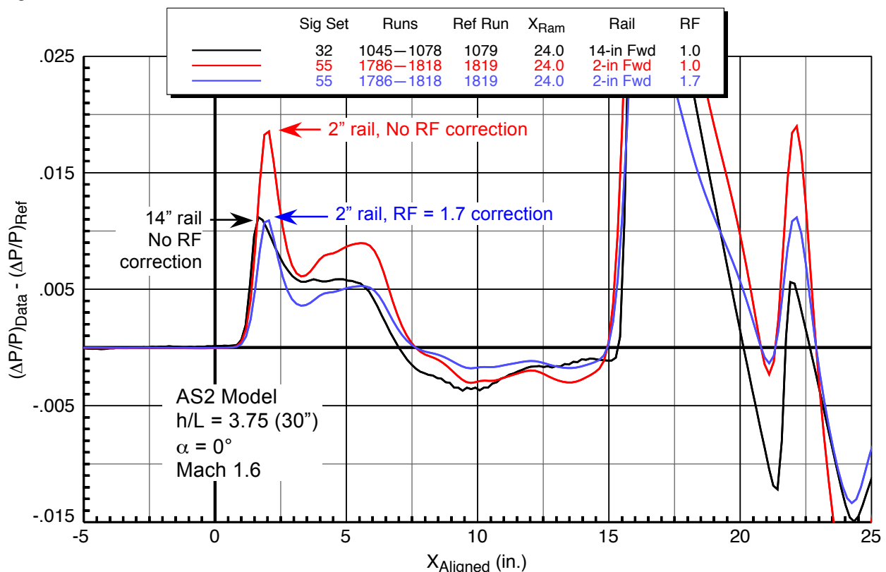
Figure 28. Rail comparisons for AS2 model, Z sweeps (26" to 34") 9x7 Parametric Test, M = 1.60 , P_T = 2293 psf, HumidAvg = 301 ppm
