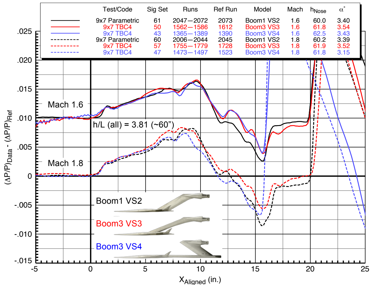
Figure 31. Boom model mounting strut effects 14-in Aft Rail, M = 1.70 , P_T = 2300 psf, HumidAvg = 244 ppm
