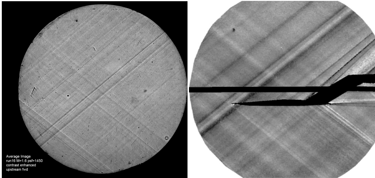
(a) Shadowgraph image, empty tunnel
