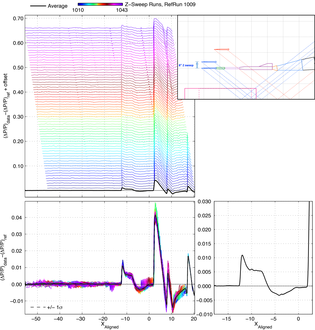
Figure 23. AS2 model aligned waterfall plot and averaged signature plots for Z sweep from 26” to 34” at X_{Ram} = 16, M = 1.6, 14” forward rail, 97p test
