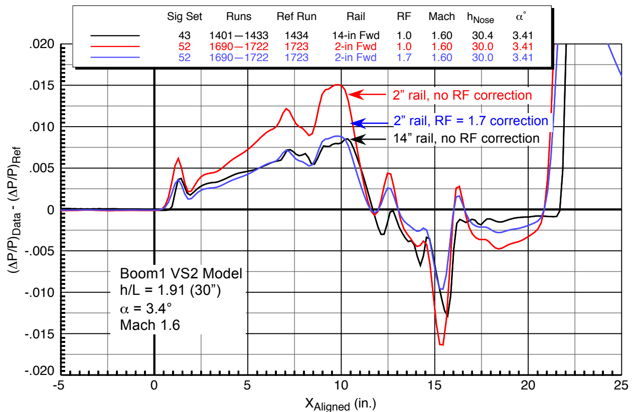
Figure 29. Rail comparisons for Boom1 VS2 model, Z sweeps (26" to 34") 9x7 Parametric Test, M = 1.60 , P_T = 2297 psf, HumidAvg = 313 ppm
