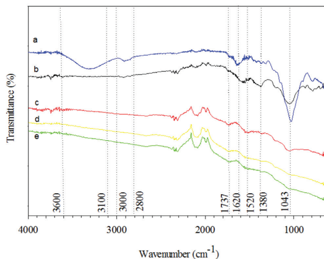
FIGURE 1. FTIR spectra of (a) RS, (b) RSC, (c) RSAC650, (d) RSAC850, and (e) RSAC750
