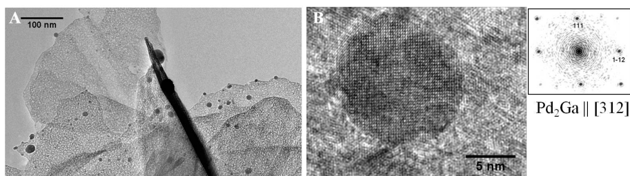
Figure 7: (A) overview TEM images PdMgGa after reduction at 773 K in 5 Vol% H 2 /Ar, and (B) HRTEM image and corresponding FFT pattern of Pd 2 Ga.
