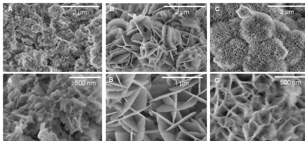
Figure 2: SEM images of (A) PdZnAl (B) PdMgGa and (C) PdMgAl HTlc precursor. (Bottom parts show magnification of top parts.)
