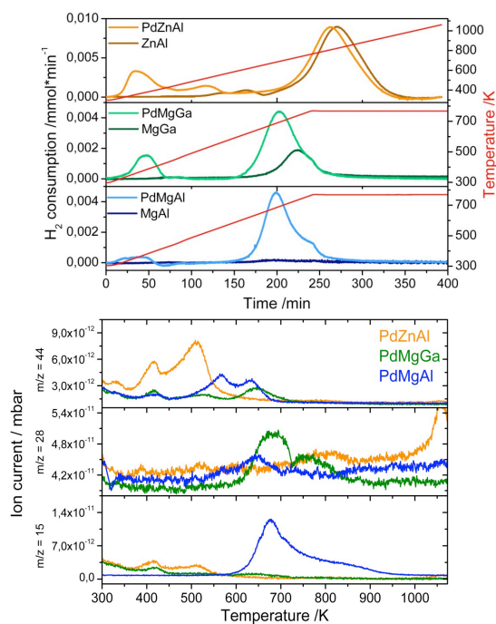
Figure 3: TPR profiles of Pd substituted and unsubstituted Hydrotalcite-like precursors (top) and MS profiles (obtained by TGA-MS) in 5 Vol% H 2 /Ar (bottom).
