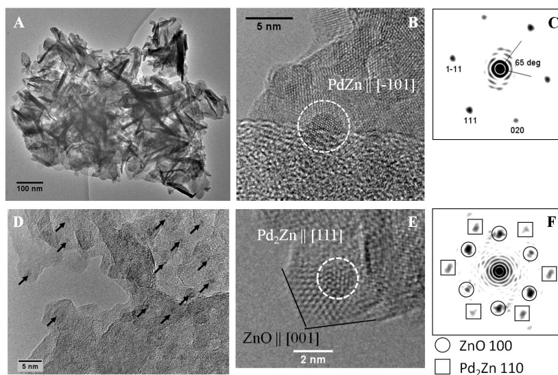
Figure 8: (A+D) Overview TEM images, and (B,E) HRTEM and corresponding FFT pattern (C, F) of PdZnAl after reduction at 523 K in 5 Vol% H 2 /Ar.
