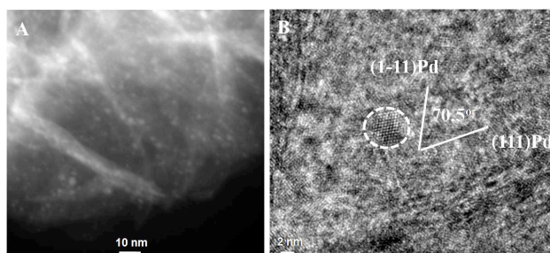
Figure 9: (A) STEM, and (B) HRTEM images of PdMgAl after reduction at 773 K in 5 Vol% H 2 /Ar.
