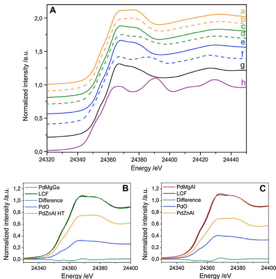
Figure 4: (A) XANES spectra PdZnAl at RT/He (a) and 323 K/H 2 (b), PdMgGa at RT/He (c) and 323 K/H 2 (d), PdMgAl at RT/He (e) and 323 K/H 2 (f), PdO (g) and Pd foil (h) reference. (B+C) Linear combination fit of the XANES spectra of PdMgGa and PdMgAl precursor, by using PdO and PdZnAl as references for Pd 2+ in square planar and octahedral coordination, respectively.
