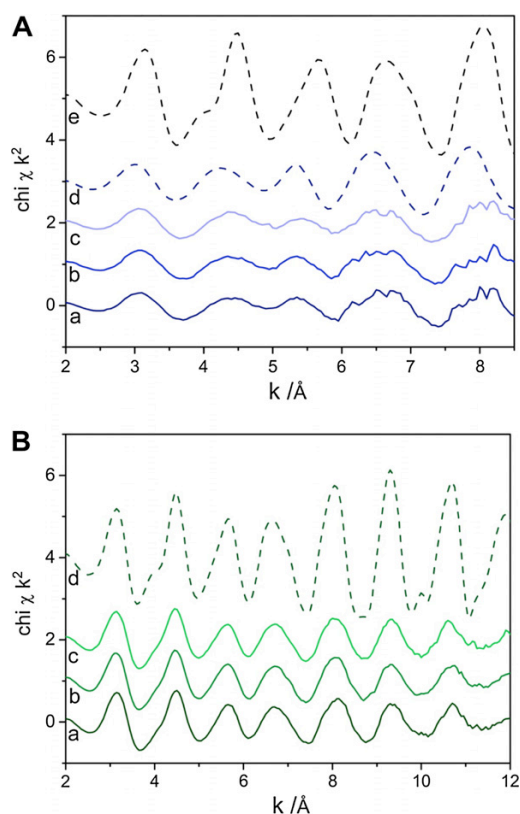
Figure 6: Pd K edge EXAFS spectra ( k^2 weighted) of PdGaMg (A) and PdMgAl (B) after reduction at 773 K (a), during MSR at 523 K (b), after 90 min MSR (c). Reference spectra are shown of bulk Pd 2 Ga (d in A) and Pd foil (e in A and d in B)
