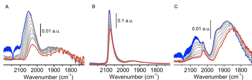
Figure 10: FT-IR spectra of CO adsorbed at room temperature on (A) PdZnAl (reduced at 523 K), (B) PdMgGa (reduced at 823 K) and (C) PdMgAl (reduced at 523 K) as a function of CO coverage ( \theta_{\max} : blue, \theta_{\min} : red).
