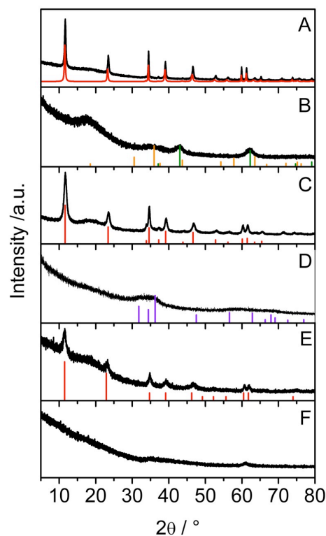
Figure 1: XRD patterns of (A) PdMgGa HTlc and simulated MgGa HTlc precursor; (B) ex- PdMgGa HTlc after reduction at 773 K, ICDD 1-1235 MgO (green), ICDD 10-113 MgGa 2 O 4 (orange); (C) PdZnAl HTlc precursor and ICDD 38-486 Zn 6 Al 2 (OH) 16 CO 3 ·4 H 2 O; (D) ex- PdZnAl HTlc after reduction at 523 K, ICDD 36-1451 ZnO (violet); (E) PdMgAl HTlc precursor and ICDD 14-191 Mg 6 Al 2 (OH) 16 CO 3 ·4 H 2 O; (F) ex- PdMgAl HTlc after reduction at 523 K.
