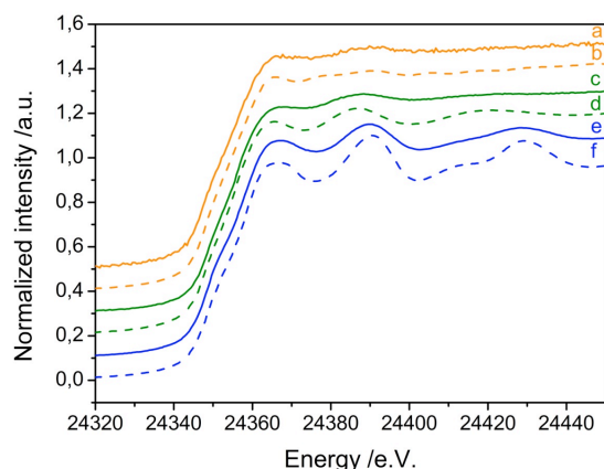
Figure 5: In situ XANES spectra of (a) PdZnAl reduced at 523 K and (b) bulk PdZn, (c) PdMgGa reduced at 773 K and (d) bulk Pd 2 Ga, (e) PdMgAl reduced at 523 K and (f) Pd foil.
