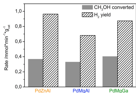
Figure 12: Rate of MSR of PdZnAl , PdMgGa and PdMgAl catalysts in MSR conducted at 523 K.
