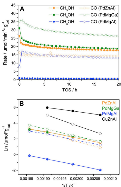
Figure 11: (A) Rate of CO 2 hydrogenation over PdZnAl , PdMgGa and PdMgAl at 523 K (30 bar, 400 mg catalyst, 100 ml/min CO 2 /H 2 ). (B) Arrhenius plot for methanol synthesis from CO 2 (closed symbols: MeOH, open symbol CO).
