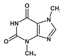
Fig. 20. Chemical structure of theobromine.
