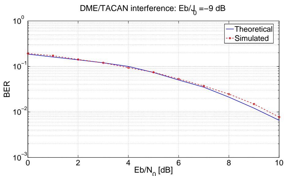
Figure 6.8: Pulse blanking impact on Bit Error Rate for un-coded DS/BPSK system in presence of AWGN pulsed interference
