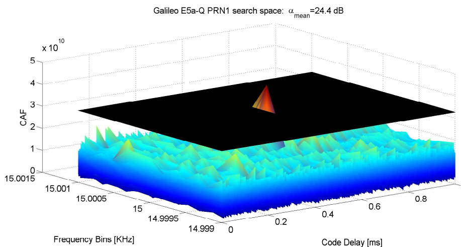
Figure 7.18: Galileo E5a-Q channel non coherent acquisition: Search Space
