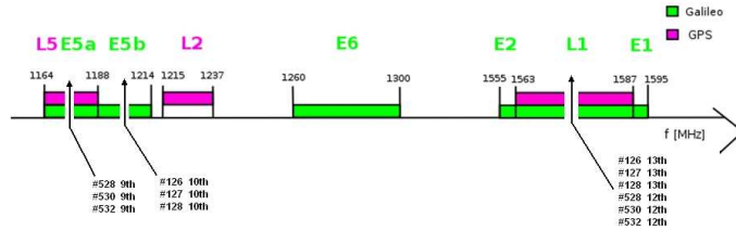
Figure 2.4: Potential VHF COM Channel Harmonic Interference.
