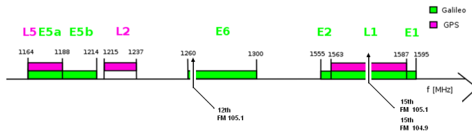
Figure 2.5: Potential FM Harmonic Interference.
