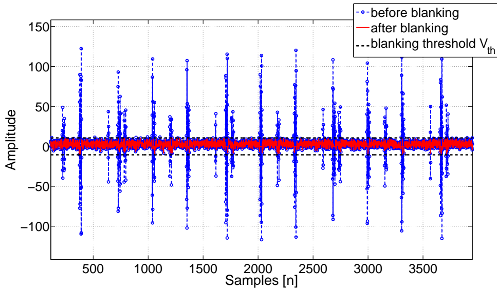
Figure 5.6: Pulse blanking applied on the single scale
