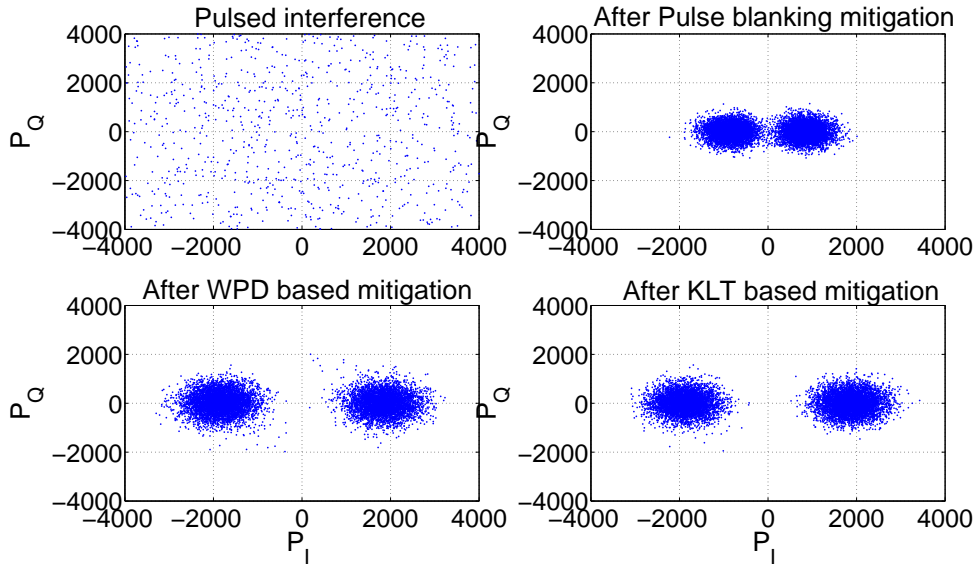
Figure 5.17: Modulation
