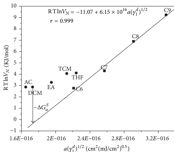
FIGURE 1: RT \ln V_N versus a\sqrt{\gamma_i^d} for n-alkanes and polar probes on PPA solid surface at 323.15 K.
