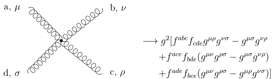
Figure 1.11: 4-Gluon Vertex
