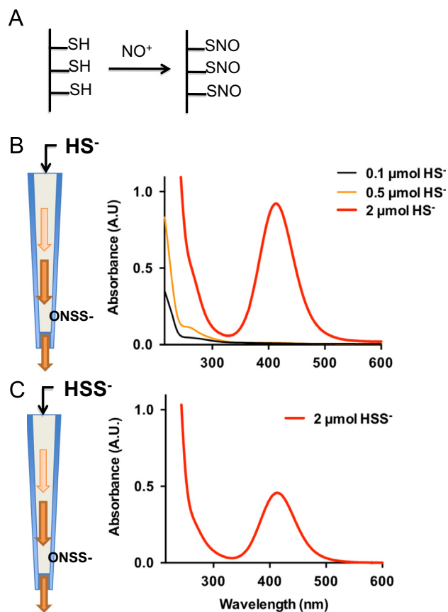
Fig. 5. Formation of \text{SSNO}^- from the reaction between sulfide and immobilized S-nitroso moieties. (A) S-nitrosation by acidified nitrite of resin-bound sulfhydryl ( -\text{SH} ) groups (Ekathiol ® ) to form an immobilized nitrosothiol. (B,C) A solution of either \text{Na}_2\text{S} (B) or \text{Na}_2\text{S}_2 (C) is passed over the column and reacts with immobilized S-nitrosothiols to form \text{SSNO}^- ( \lambda_{\text{max}} 412 nm; high sulfide concentration) and polysulfides ( < 280 nm; lower sulfide concentrations). Depicted results are representative of 4 independent experiments with different batches of nitrosated thiol-containing resin and various absolute amounts of sulfide (0.015–5 \mu\text{moles} on column).
