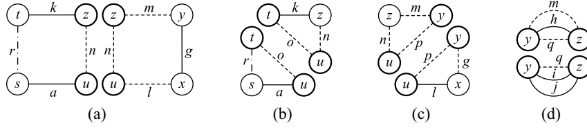
Fig. 4. (a) A split of a hexagon from Fig.3(b), (b)-(c) a split of a tetragon, (d) a split of a bond The graphs formed by the sets E_0 \cup \{e\} and E_1 \cup \{e\} are the obtained split graphs of the performed split operation. A virtual edge is visualized by a dashed line.
