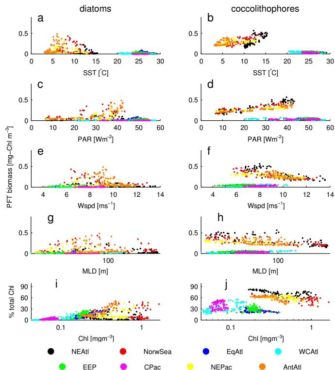
Fig. 3. Scatter plots showing the emerging relationship between PhytoANN diatom (left column) and coccolithophore (right column) biomass [ \text{mg Chl m}^{-3} ] (a–h) or % of total Chl (i, j) vs. individual ecological indicators color coded according to domain of origin. On the x-axis from top to bottom: SST, PAR, Wspd, MLD, Chl. All data points come from exploratory analysis only, thus they are box-average and monthly average estimates from October 1997 to December 2004.
