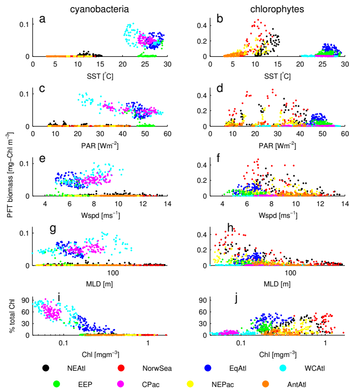
Fig. A2. Scatter plots showing the emerging relationship between NOBM cyanobacteria (left column) and chlorophyte (right column) biomass [ \text{mgChl m}^{-3} ] (a–h) or % of total Chl (i, j) vs. individual ecological indicators color coded according to domain of origin. On the x-axis from top to bottom: SST, PAR, Wspd, MLD, Chl. All data points come from exploratory analysis only, thus they are box-average and monthly average estimates from October 1997 to December 2004.
