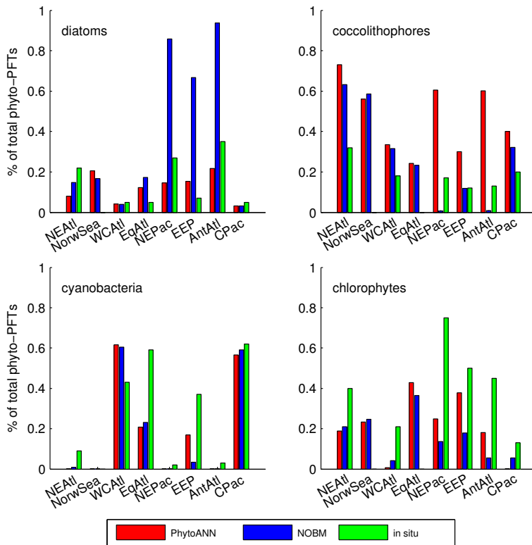
Fig. 6. Approximate box or basin-average comparison between longterm (1997–2004) annual mean percentage contribution to total Chl biomass of diatoms, coccolithophores, cyanobacteria and chlorophytes according to NOBM (blue), PhytoANN (red) and in situ (green) estimates. In situ estimates were derived from both C- and Chl-based measurements. Here, estimates were derived from a combination of data collected by Gregg et al. (2003) ( http://gmao.gsfc.nasa.gov/research/oceanbiology/data.php ) and EEP data from Taylor et al. (2011, their Table 3).
