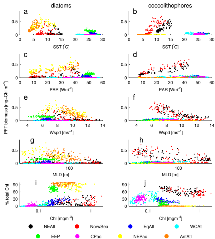
Fig. A1. Scatter plots showing the emerging relationship between NOBM diatom (left column) and coccolithophore (right column) biomass [ \text{mgChl m}^{-3} ] (a–h) or % of total Chl (i, j) vs. individual ecological indicators color coded according to domain of origin. On the x-axis from top to bottom: SST, PAR, Wspd, MLD, Chl. All data points come from exploratory analysis only, thus they are box-average and monthly average estimates from October 1997 to December 2004.
