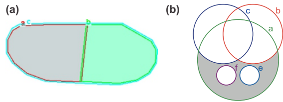
Figure 3: (a) A well-matched Euler diagram that is not well-formed and whose curves are not smooth [RZF08], and (b) a not well-matched Euler diagram with shading that is well-formed and has smooth curves [SFRH12].
