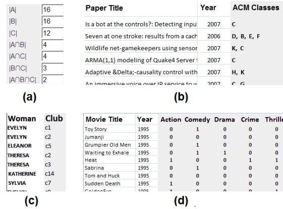
Figure 2: Various forms of set-typed data: (a) the cardinality of set relations, (b) a multi-valued attribute (in grey), (c) a membership list, (d) Boolean attributes (in grey).
