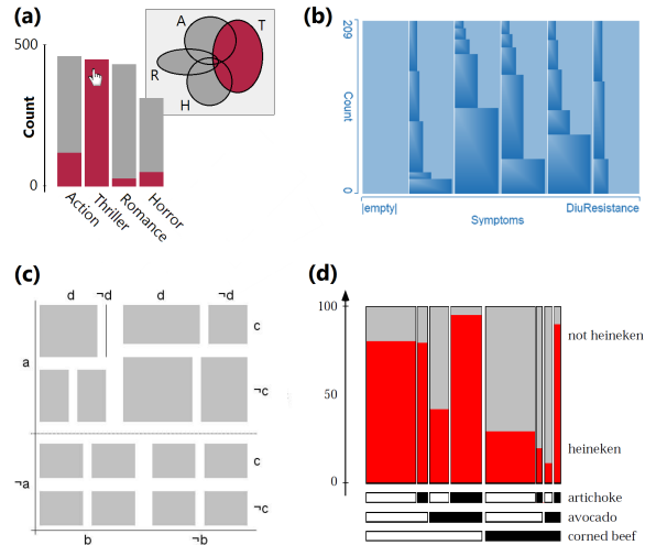
Figure 14: Aggregation-based techniques: (a) an interactive bar chart [AAMH13], (b) Set’o’gram [FMH08], (c) Mosaic displays [Hof00], (d) Double-Decker plot [HSW00].
