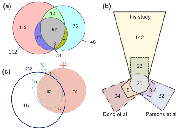
Figure 5: Area-proportional Venn diagrams drawn with: (a) circles [MM11] using Venn Diagram Plotter [LM13]; (b) polygons [RGSB*11] using 3 Circle [CR05b]; (c) ellipses using eulerAPE [MR14] for the numeric data in (a).
