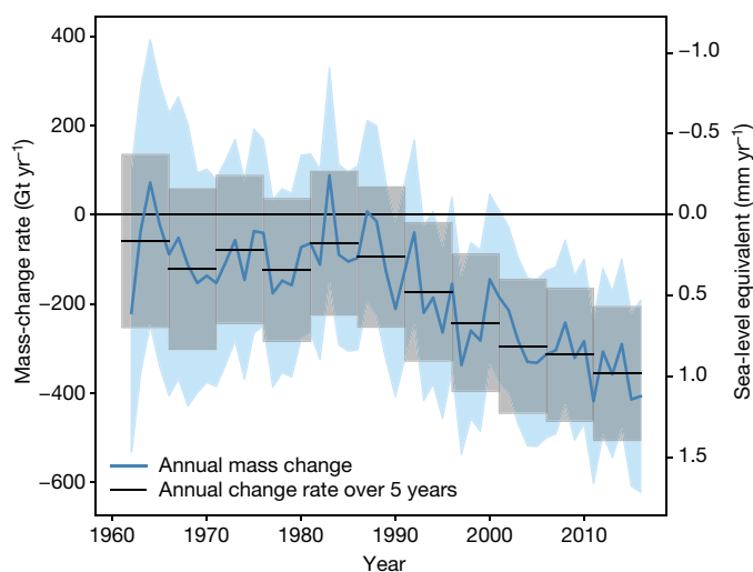
Fig. 2 | Global glacier contributions to sea-level rise from 1961 to 2016. Annual and pentadal mass-change rates (left vertical axis) and equivalents of mean global sea-level rise (right vertical axis) are shown with related error bars (indicated by shading) corresponding to 95% confidence intervals. Annual errors originate from independent sources: glaciological sample, geodetic sample, spatial interpolation and glacier area. Over the five-year periods, the individual error terms are cumulated separately and then the multiyear terms are combined according to the law of random error propagations, and divided by the number of years (see Methods).
