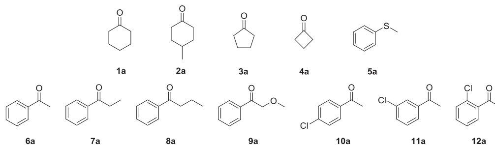
Fig. 3. Panel of substrates studied in this work. Substrate 5a for Tm CHMO can be oxidized to methyl phenyl sulfoxide ( 5b ) or to (methylsulfonyl)benzene ( 5c ).
