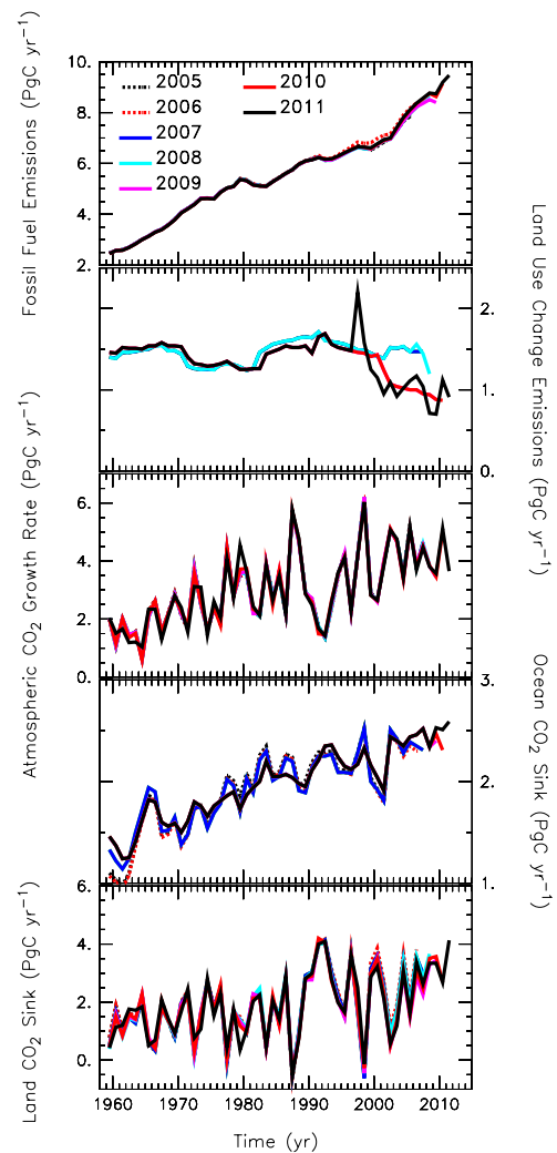
Figure 6. Comparison of global carbon budget components released annually by GCP since 2005. CO 2 emissions from both (a) fossil fuel combustion and cement production, and (b) land-use change, and their partitioning among (c) the atmosphere, (d) the ocean, and (e) the land. The different curves were published in (dashed black) Raupach et al. (2007), (dashed red) Canadell et al. (2007), (dark blue) online only, (light blue) Le Quéré et al. (2009), (pink) Friedlingstein et al. (2010), (red) Peters et al. (2012a), and (black) this study. All values are in PgC yr -1 .
