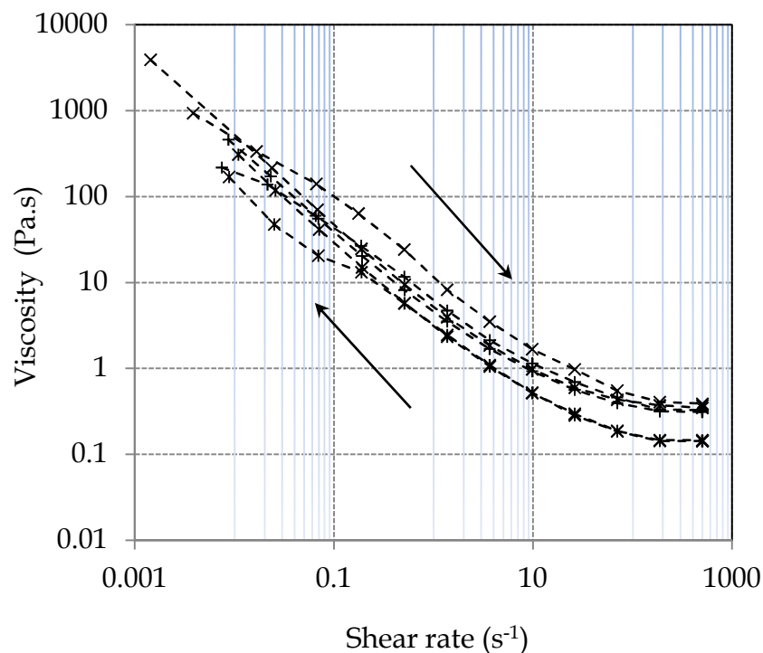
Figure 53: Example of thixotropic hysteresis loop of composites 80%Ca-HA/20%(G) and 80%Ca-HA/20%(P) (---*---Ca-HA Gel ( \eta_{\infty}=0.144\text{Pa.s} ),--x-- 80%Ca-HA Gel /20%(P) ( \Gamma=0.369 ; \eta_{\infty}=0.348\text{Pa.s} ), --+--80%Ca-HA Gel /20%(G) ( \Gamma=0.384 ; \eta_{\infty}=0.318\text{Pa.s} )
