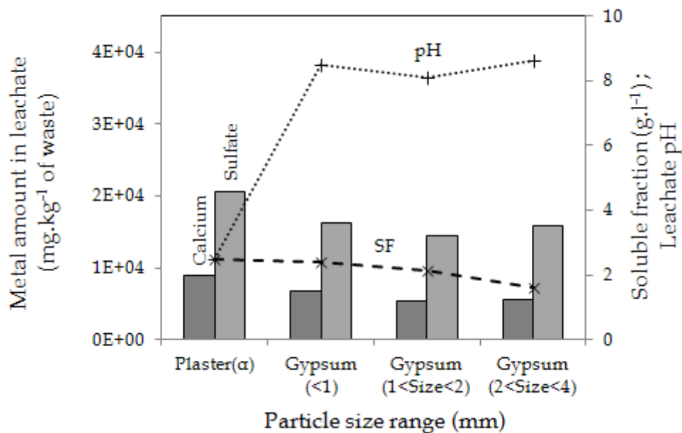
Figure 66 : Leachability of calcium and sulfate from plaster, gypsum (<1mm), gypsum (1-2mm) and gypsum (2-4mm) as a function of the leachate pH (after 48 h of tumbling at 7 rpm) and soluble fraction (SF)
