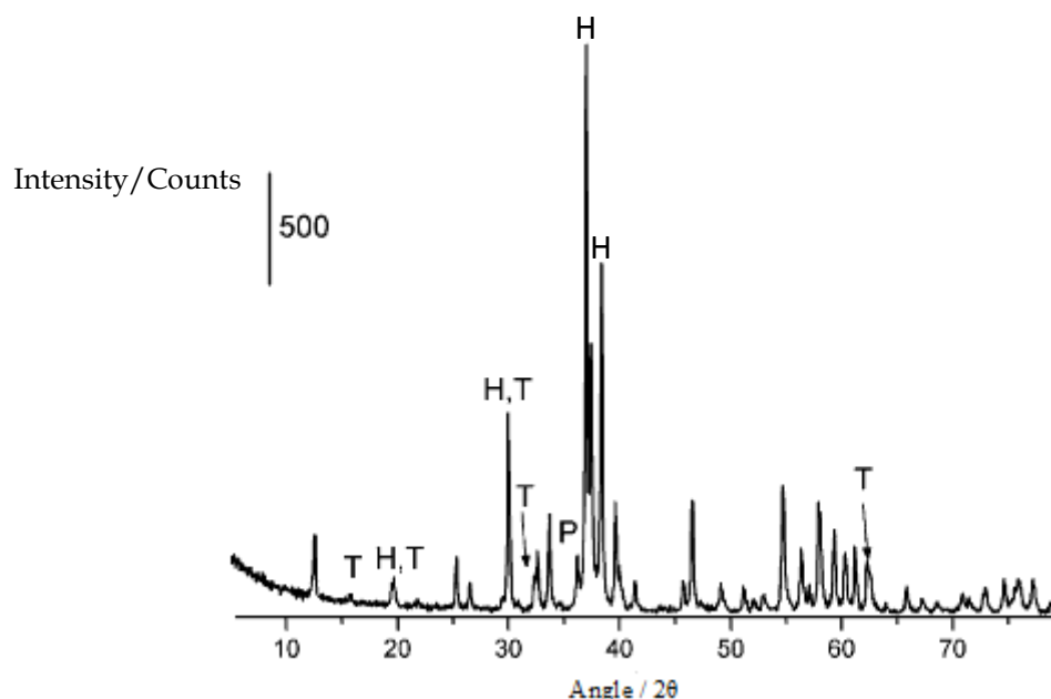
Figure 9: Diffraction pattern of hydroxyapatite after heat treatment [60] H is the tribasic calcium phosphate (Ca-HA), \text{Ca}_5(\text{PO}_4)_3(\text{OH}) , T corresponds to tricalcium phosphate ( \alpha -TCP), \text{Ca}_3(\text{PO}_4)_2 and P is the tetracalcium phosphate (TCPM), \text{Ca}_4(\text{PO}_4)_2\text{O} .
