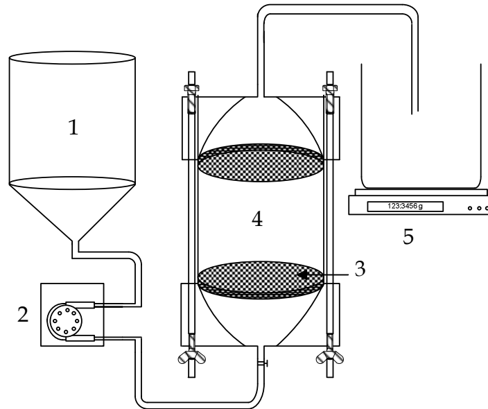
Figure 80: Percolation test system (1: reservoir, 2: peristaltic pump, 3: filter system, 4: permeametric cell, 5: weighing)
