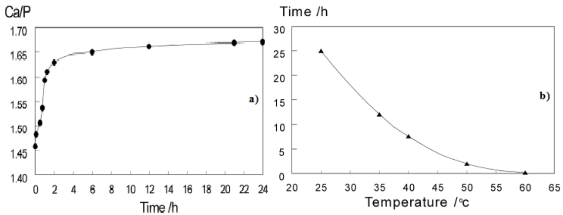
Figure 6: a) Variation of the ratio Ca/P as a function of reaction time at 35°C, b) Formation time of pure Ca-HA as a function of temperature according to Lui et al (2001) [52]
