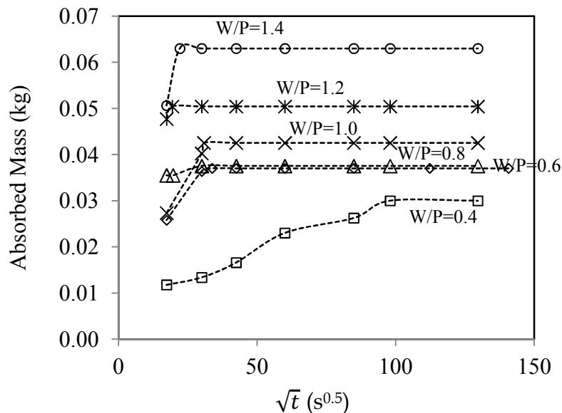
Figure 38 : Adsorbed mass in plaster specimen body as a function of time square
