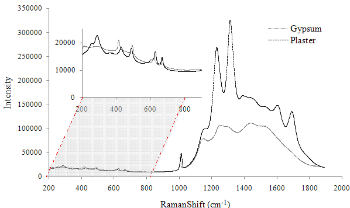
Figure 30 : Raman spectra of gypsum and plaster ( \alpha ) under ambient conditions
