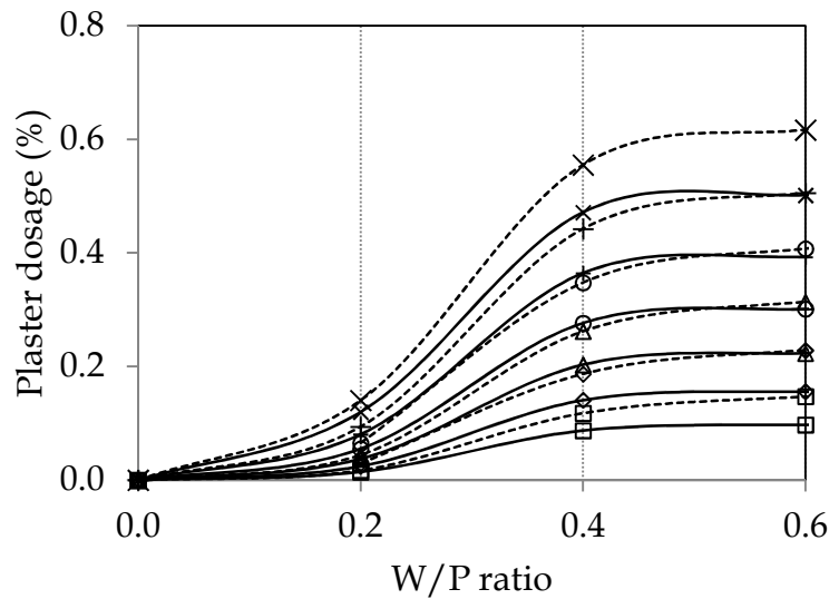
Figure 41: Hydrated plaster dosage in function of W/P ratio
