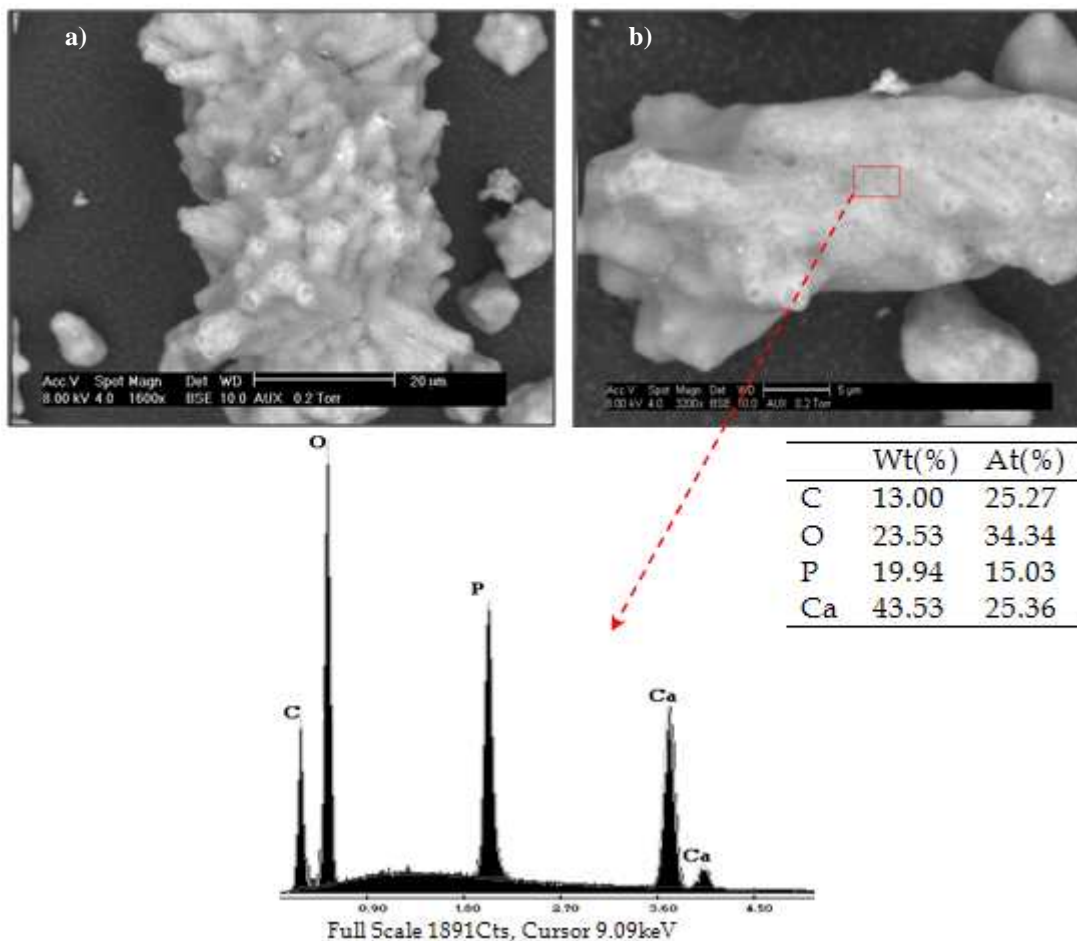
Figure 21 : ESEM of Ca-HA dried at 105°C (5-20μm)
