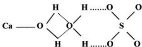
Figure 32 : Proposed structure of gypsum according to Mandel et al. (2002) [9]
