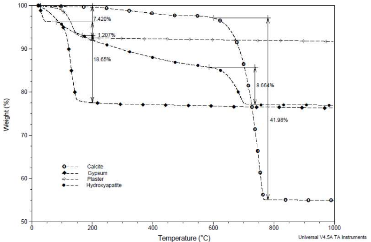
Figure 28: Thermogravimetric analysis of calcite, gypsum, plaster ( \alpha ) and Ca-HA Powder
