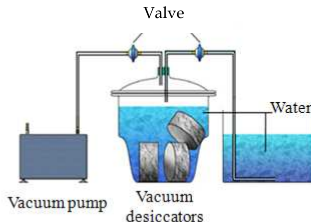
Figure 36 : Water porosity test
