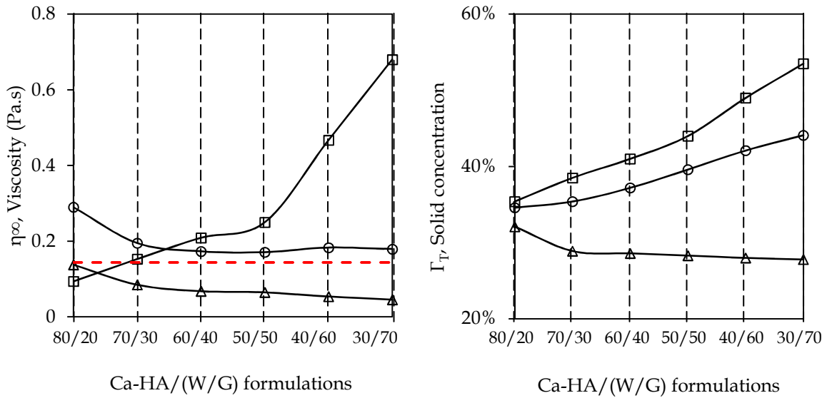
Figure 55: Variation of viscosity of Ca-HA/(W/G) mixtures at different mass ratios (— Ca-HA Gel (0.144Pa.s), —□— Ca-HA/(W/G=0.2), —○— Ca-HA / (W/G=0.4), —Δ— Ca-HA/(W/G=0.6))
