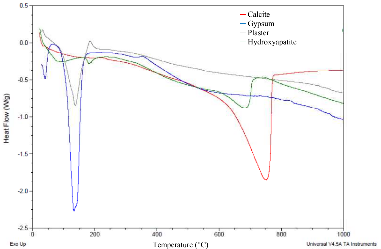
Figure 27 : Differential scanning calorimetry of calcite, gypsum, plaster and Ca-HA Powder
