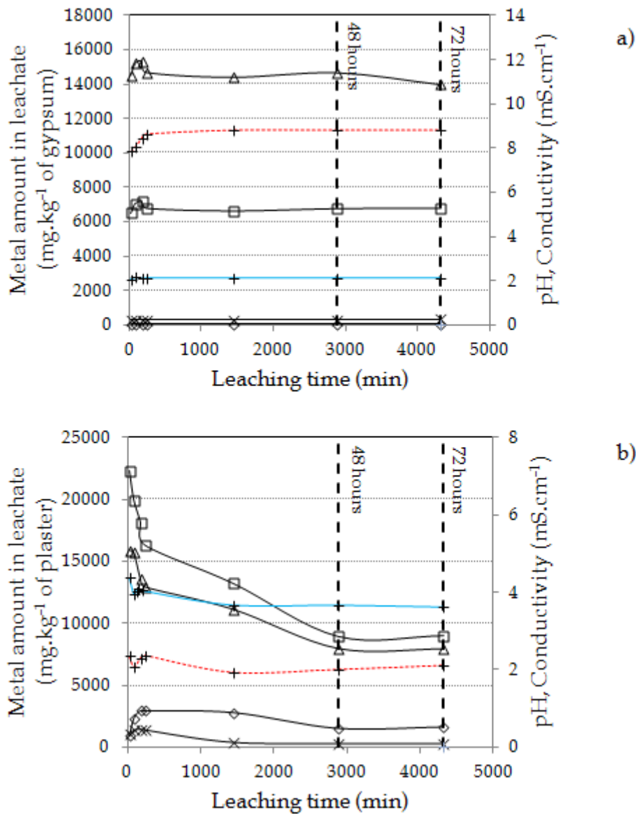
Figure 65 : The effect of leaching duration on the leachability of calcium (—□—), sulfur (—Δ—), phosphorus (—◇—) and strontium (—×—) from a) gypsum and b) plaster (···+··· pH, —+— Conductivity (mS.cm -1 ))
