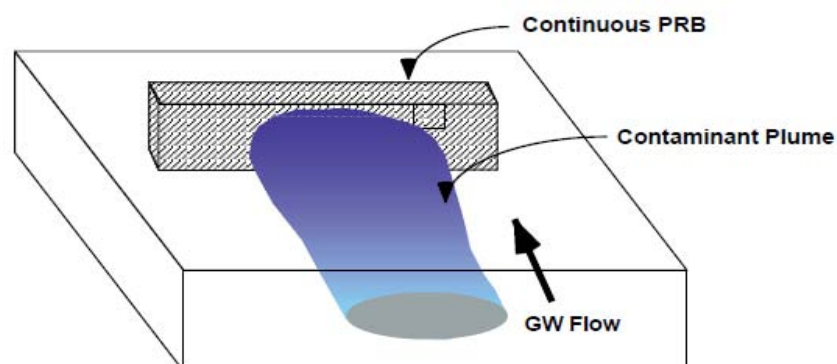
Figure 2 : Continuous PRB trenched system [12]
