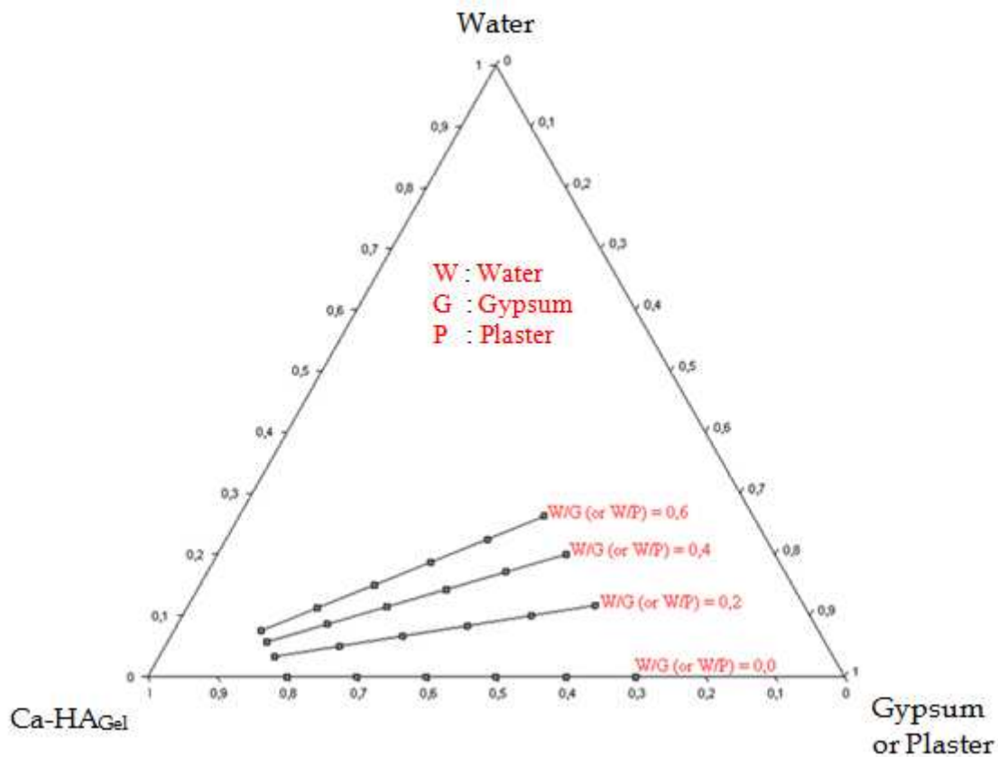
Figure 39: Ternary phase diagram showing different mixtures of Ca-HA Gel , Gypsum (<1mm) and plaster
