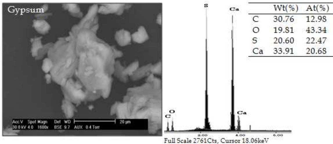
Figure 19 : SEM picture and EDS analysis corresponding to gypsum (<1mm) (20μm)
