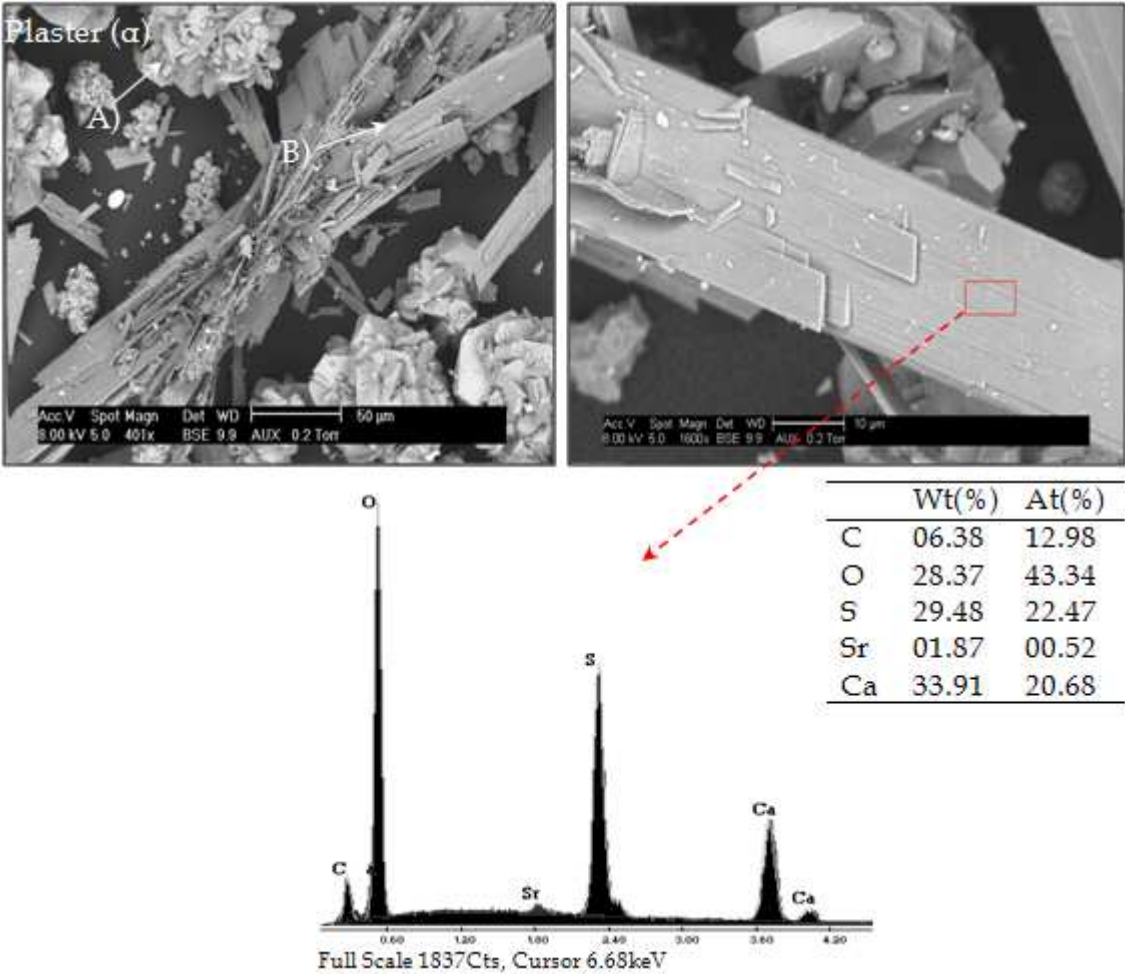
Figure 18 : SEM pictures of plaster (α) (10-50µm)
