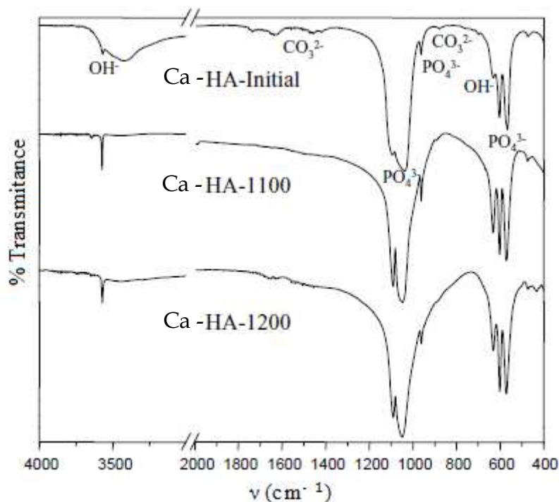
Figure 8: IR spectrum of hydroxyapatite calcined at different temperatures according to PADILLA et al (2005) [56]
