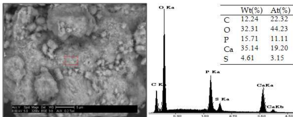
Figure 45 : Environmental SEM of 80%Ca-HA/20%(W/P=0.4) formulation
