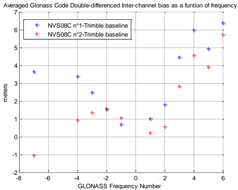
Figure 2.13 Averaged code GLONASS double-differenced inter-channel bias, for 2 distinct NVS08C connected to the same antenna. Double-differences are formed with TLSE (Trimble receiver) observations for both receivers.
