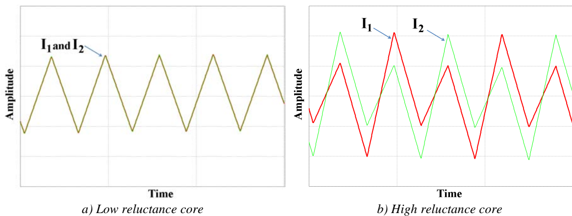
Figure III.3: Currents in the two phases of an ICT.
