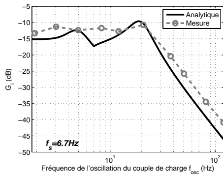
(a) f_s = 6.7 \text{ Hz}
