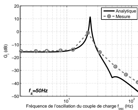
(e) f_s = 50 \text{ Hz}
