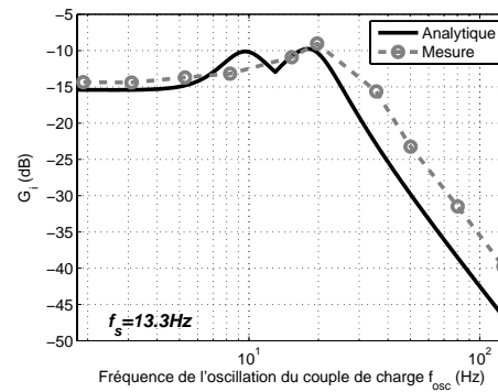
(b) f_s = 13.3 \text{ Hz}
