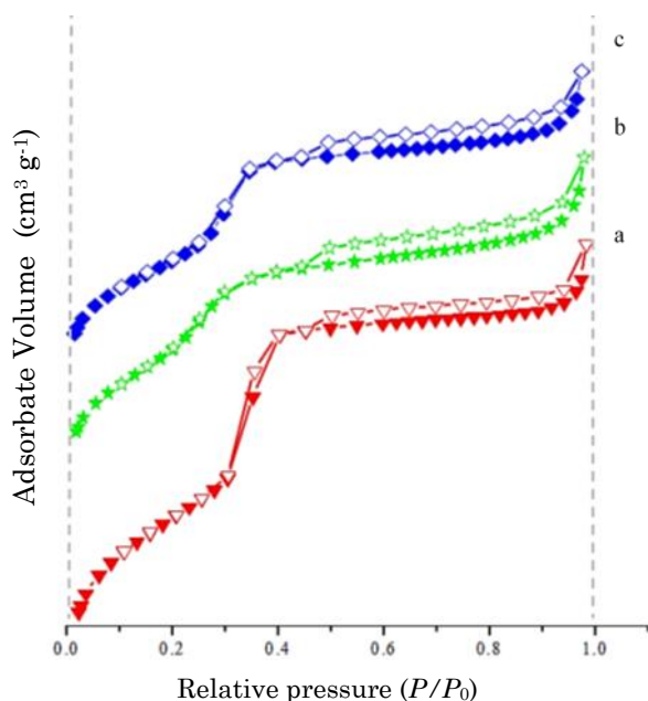
Figure 2. N_2 adsorption-desorption Isotherm of samples a. A-6-70, b. A-12-70, c. A-24-70
