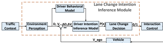
Fig. 3. Driver lane change intention inference framework.
