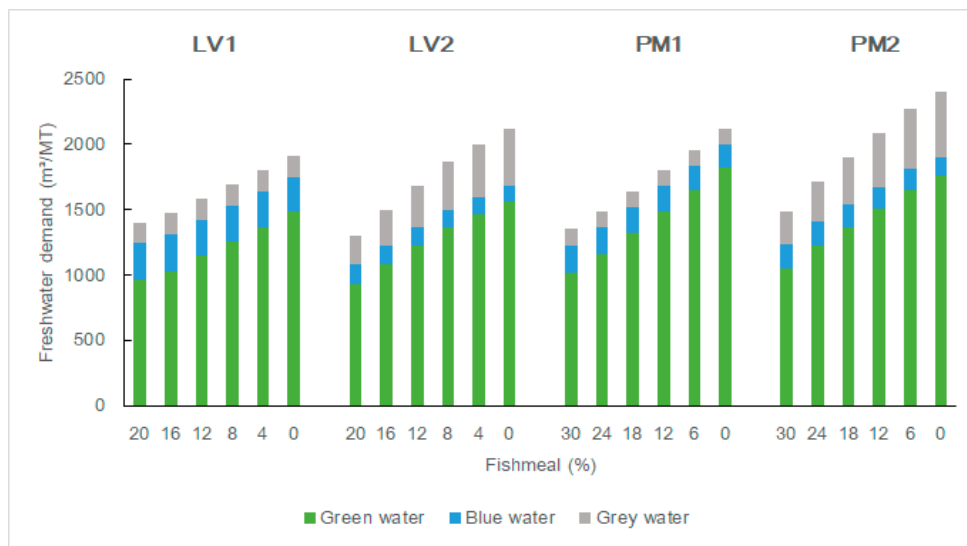
Figure 1. Freshwater demand (m 3 /MT) for the baselines and five substitution levels in two scenarios and for two species. Green bar indicates consumed rainwater, blue bar indicates consumed or evaporated volume of surface and groundwater (irrigation), and grey bar indicates freshwater needed to process and neutralize pollutants.
