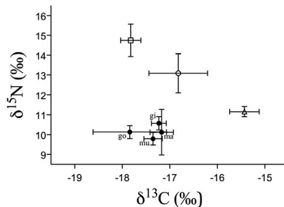
Fig. 2. – Mean ( \pm sd) \delta^{13}\text{C} and \delta^{15}\text{N} values of the carapid fish Onuxodon fowleri (white square), the palaemonid shrimp Conchodytes meleagrinae (white circle), zoobenthos (white triangle), and tissues of the black-lip pearl oyster Pinctada margaritifera (black circles) from Makemo Atoll (Tuamotu Archipelago, French Polynesia); gi, gills; go, gonads; ma, mantle; mu, muscles.
