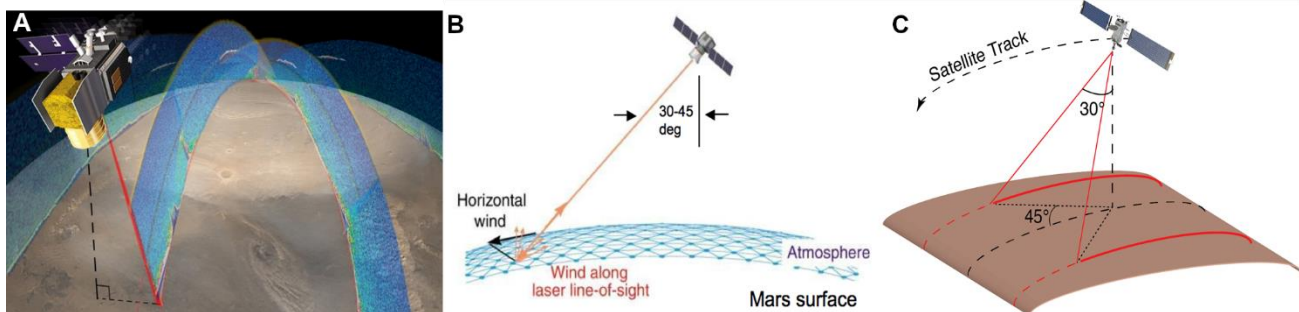
Figure 2. MARLI measurement concept. (A) Conceptual drawings of the MARLI instrument in a Mars polar orbit. (B) Off-nadir measurement concept for scalar wind measurement along lidar line-of-sight (LOS). (C) A dual-beam concept of the instrument, which allows vector wind measurements.
