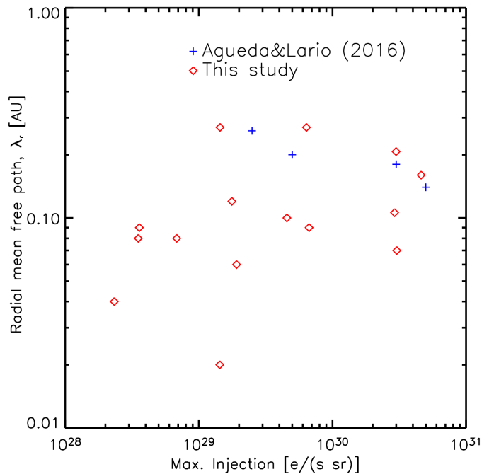
Fig. 9. Radial mean free path vs. maximum electron injection at the Sun, i.e. the highest injection inferred for each event as shown in Figs. 6–8. Diamonds: values inferred in this study; crosses: values from Agueda & Lario (2016) .
