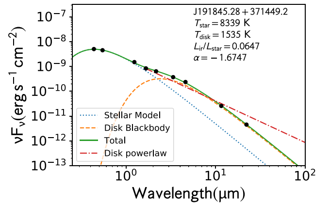
Figure 8. SED for WISEA J191845.28+371449.2. This system is well fit by a stellar temperature blackbody with a \sim 1535 \text{ K} disk blackbody with fractional infrared luminosity \sim 0.065 , suggesting an extreme debris disk.
