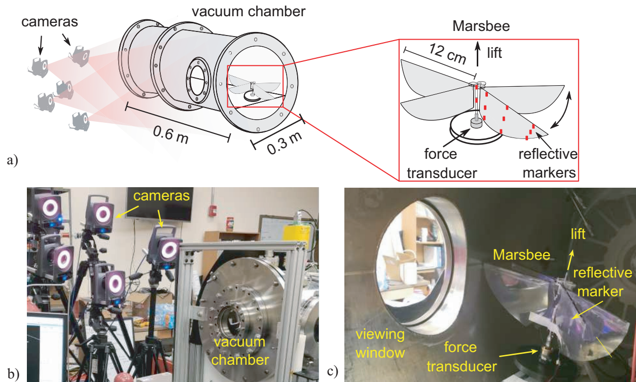
Figure 21. Marsbee experimental setup in the smaller vacuum chamber. a) Schematic of vacuum chamber and motion tracking cameras. b) Outside view of the vacuum chamber with the Vicon motion tracking cameras looking through the chamber’s side viewing window. c) Interior view of the vacuum chamber housing the Marsbee test stand.
