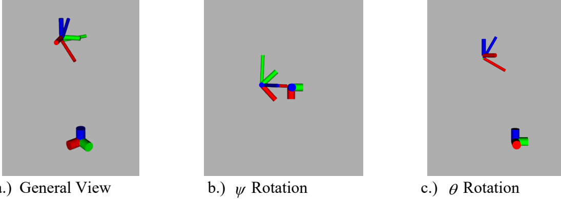
Figure 38. The three frames are shown with three axes (red: first axis, green: second axis, blue: third axis). The Mars frame (short and thick) is fixed to the planet. The body-fixed frame (medium thickness and length) is fixed to the camera frame (long and narrow). The rotation of \psi (b) represents the fixed camera yaw rotation and \theta (c) represents the downward angle of the camera to capture the surface of Mars below the flying robot.
