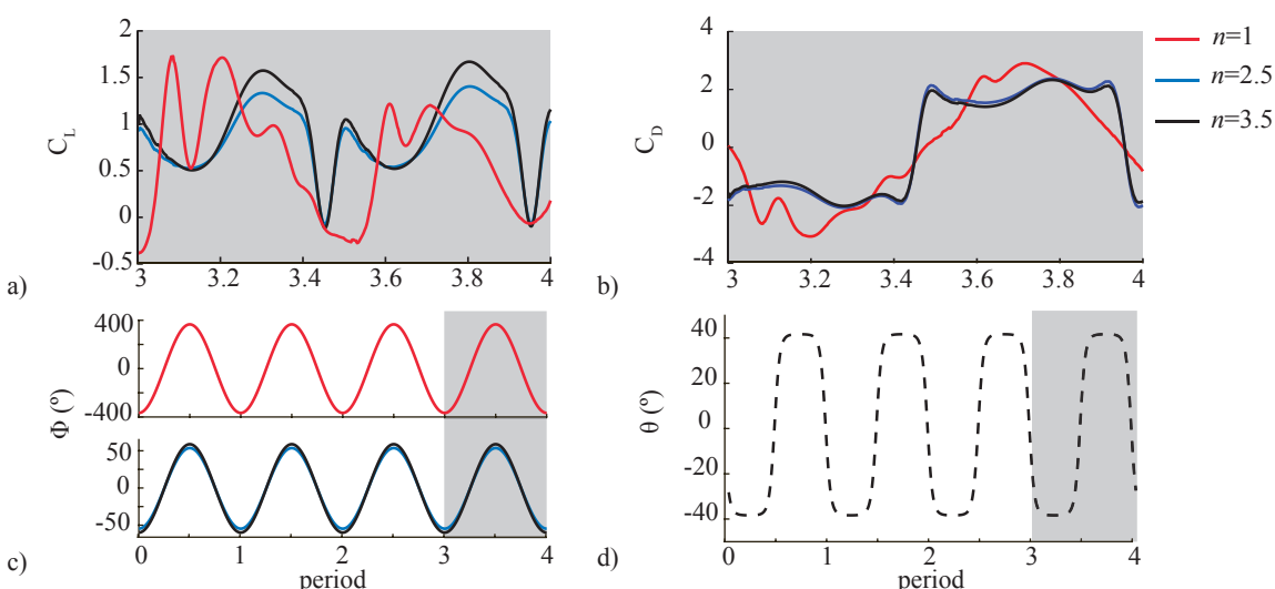
Figure 11. a) Lift and b) drag produced by a bee on Mars ( n=1 ) and two bumblee-sized Marsbees ( n=2.5 and n=3.5 ) during the fourth and final flapping period. Corresponding c) flapping and d) pitching motions, where the flapping amplitude varies as a function of n while the pitching amplitude is the same for all values of n .
