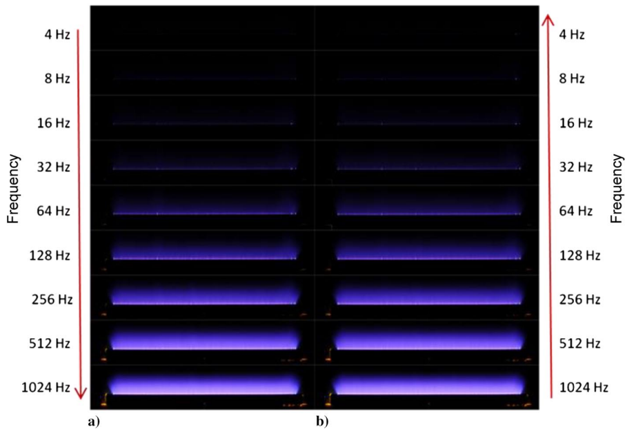
Fig. 8 Images of discharges corresponding to Fig. 7, 48 kV p-p frequency sweep.
