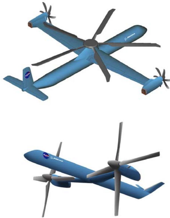
Figure 9.4. Large transport rotorcraft reference designs used for conducting a technology benefits assessment (Wilkerson and Smith [2009]).
