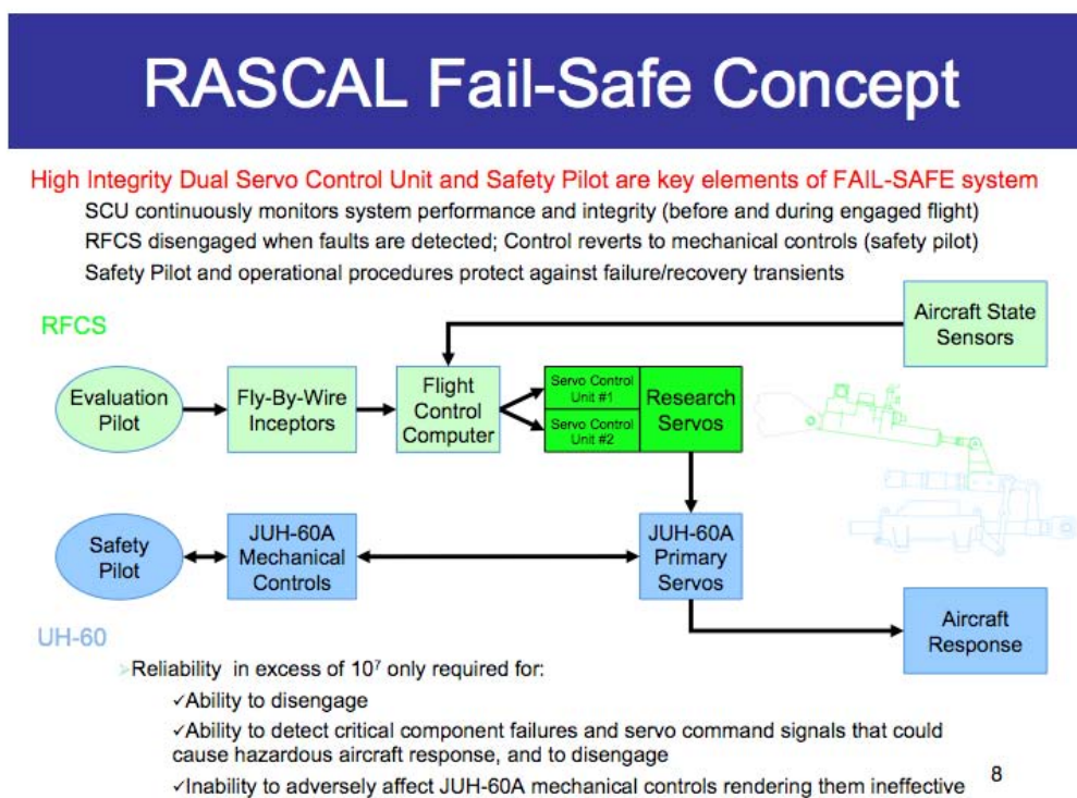
Figure 6.9. U.S. Army/NASA RASCAL fail-safe concept.
