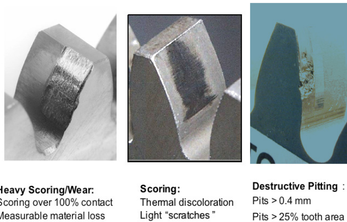
Figure 7.10. Conceptual gear failure mechanism map.
