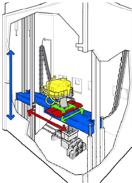
Figure 6.3 Cutaway diagram of the VMS facility.
