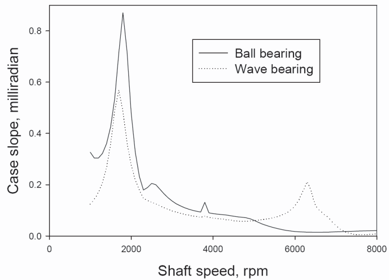
Figure 3.20. Angular vibration of transmission case for 28 \times excitation.
