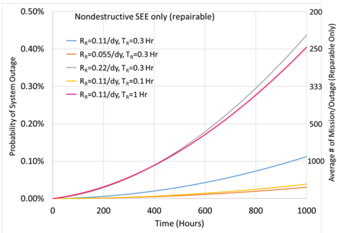
Figure 12. Outage Probability as a Function of Repairable SEE Rate and Repair Time
