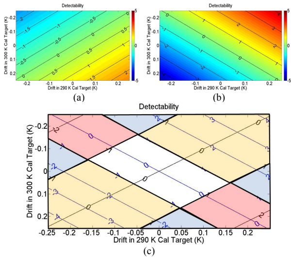
Fig. 7. (a) Detectabilities from the measurement mode (Figure 4-b). (b) Detectabilities from the calibration validation mode (Figure 6-b). (c) Calibration error analysis (CEA) diagram combining (a) and (b).
