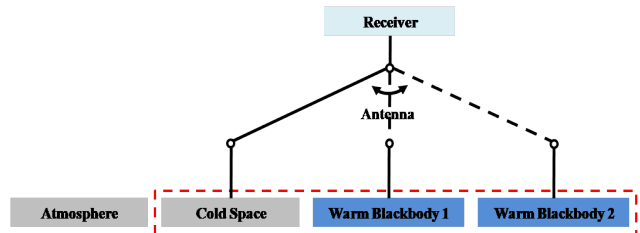
Fig. 5. Radiometer with three calibration targets in calibration validation mode. Atmosphere is not measured, cold space is calibrated using two blackbody targets.
