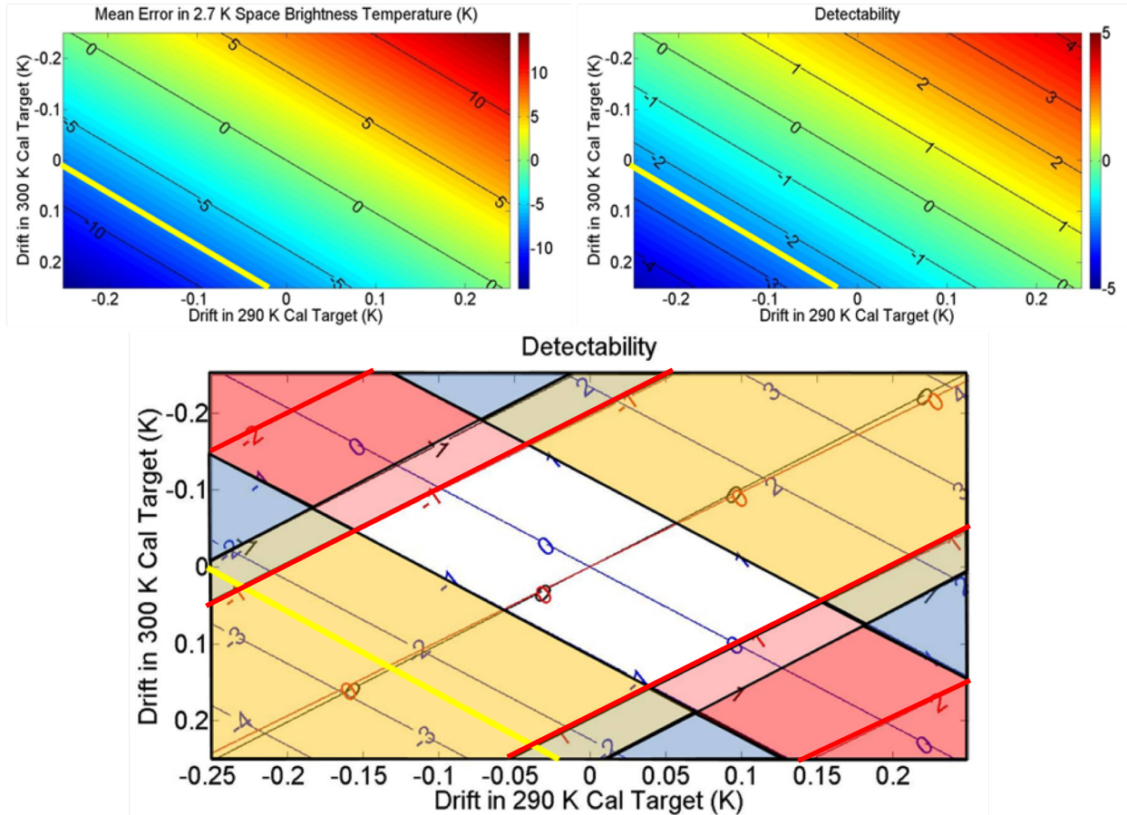
Fig. 9. (top-left) 7.5 K error detected in cold space measurements during the calibration validation mode. (top-right) Detectability of the error. (bottom) The error in the CEA diagram. Notice that if the atmosphere is cold, the entire line is within the yellow region where the impact of the calibration drift on the atmospheric measurements is minimal during the measurement mode.
