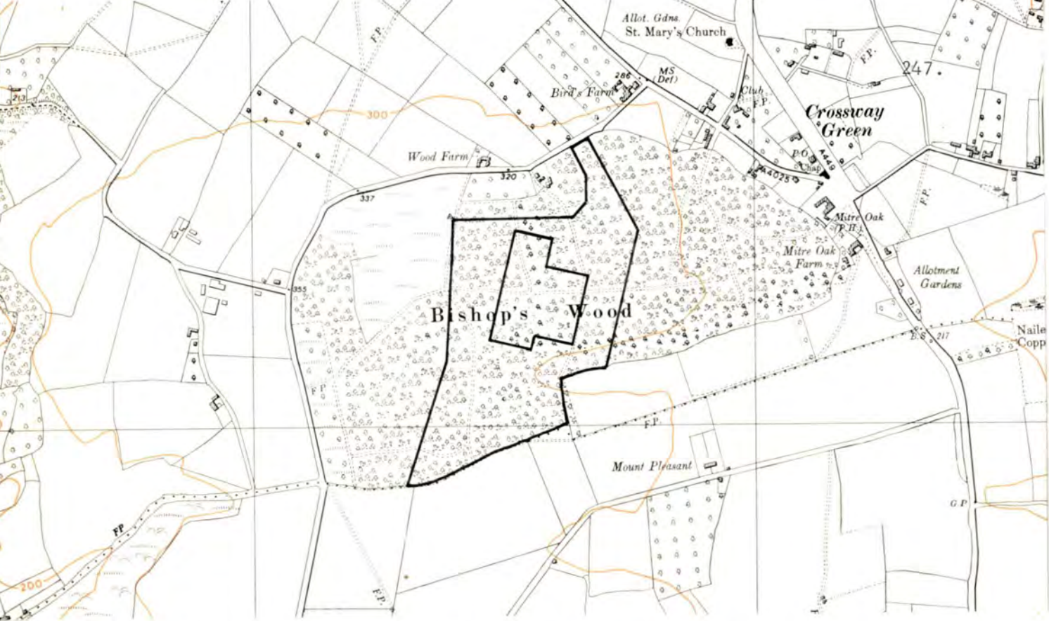
Map 45 showing location of Bishop's Wood 275/132 kV substation, Worcestershire which although sited on the crest of a small hill is effectively screened from all the nearby houses.
