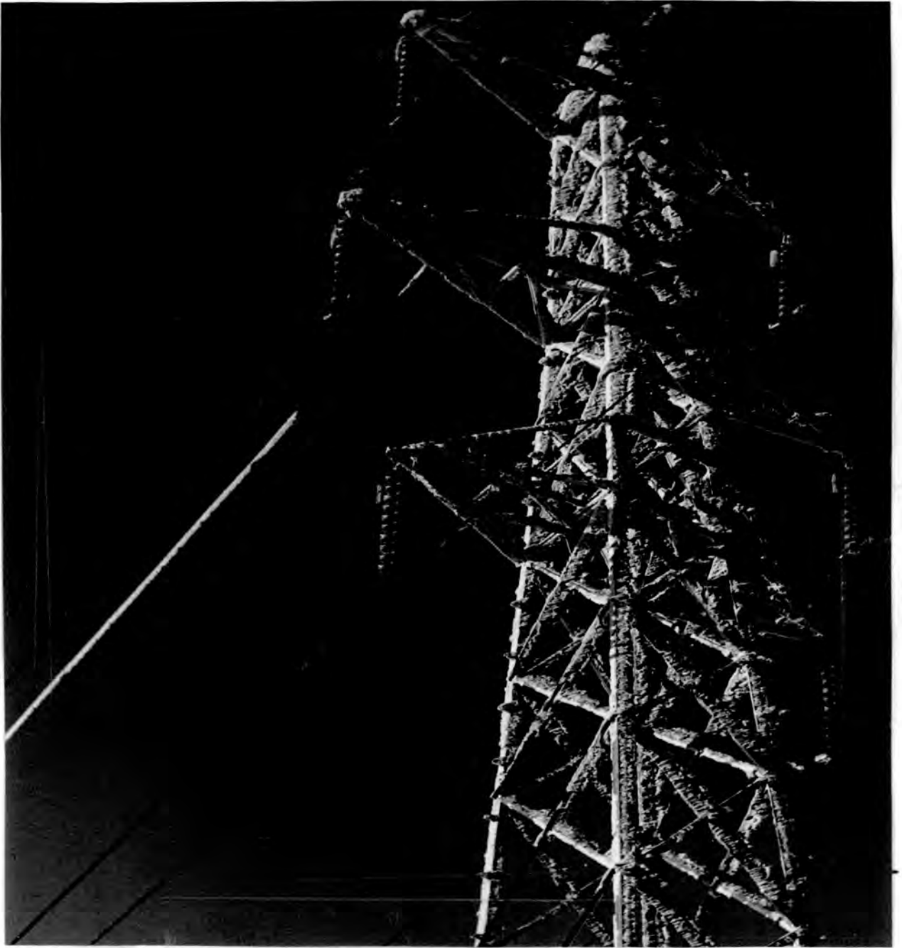
Photograph 4. Icing on the Uskmouth to Crumlin Llantarnam 132 kV line.
