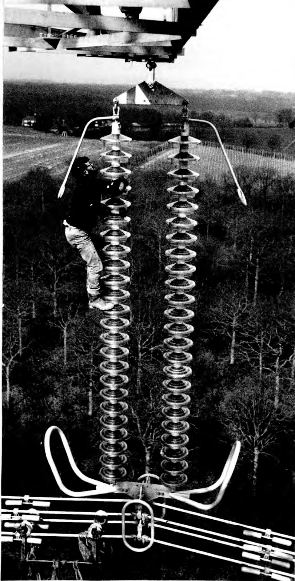
Photograph 65. A suspension string of glass insulators on a 400kV line. The trolley with which the linesman inspects the conductors and insulators is just visible in the bottom left hand side of the photograph.
