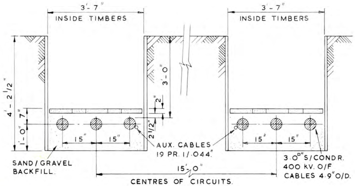
Drawing 4. Normal trench cross section for 400 kV cable installation at Streatley, Berkshire (62)
