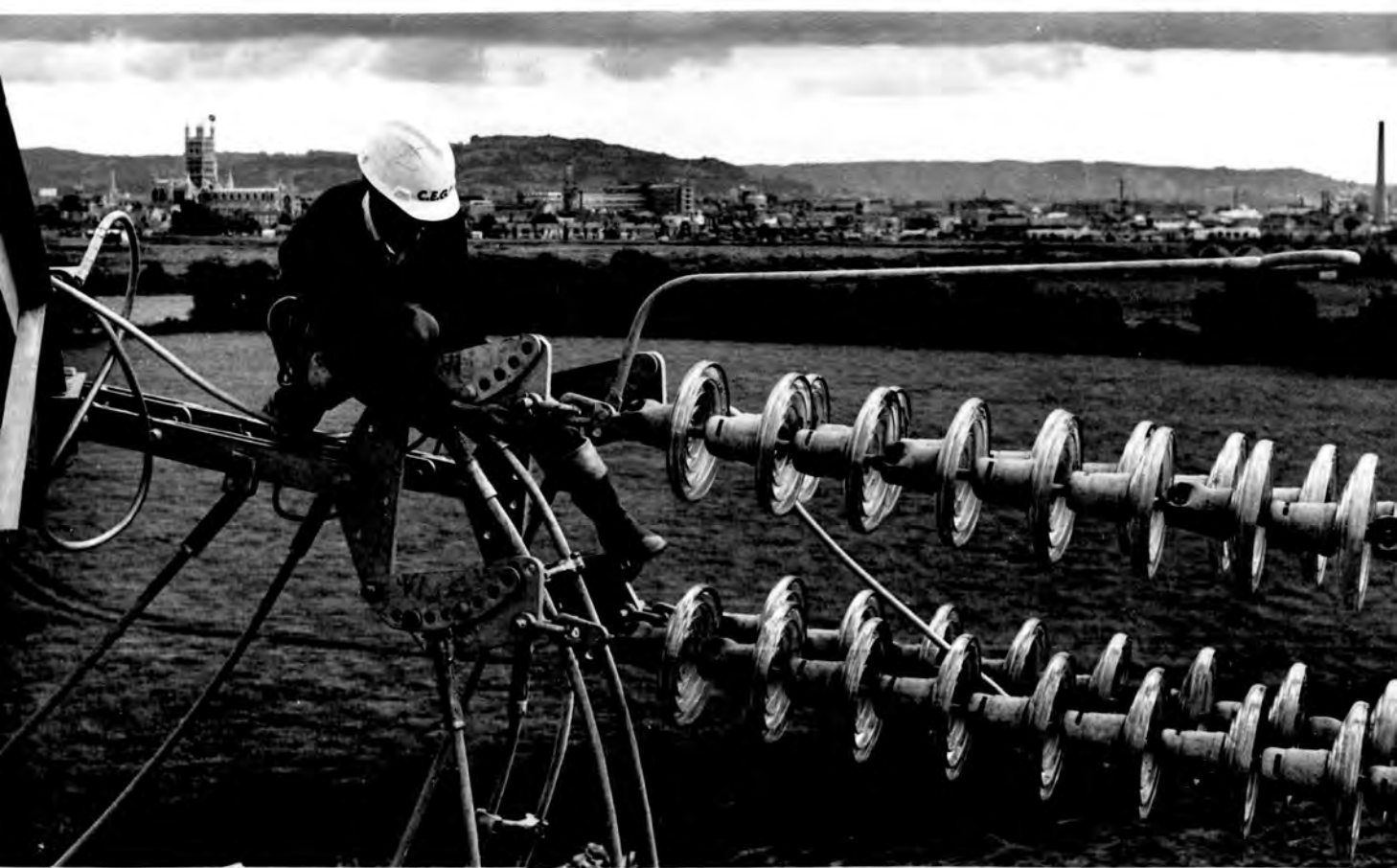
Photograph 66. A tension string of four, 400kV glass insulators, at the Gloucester end of the line to Ystradgynlais substation in South Wales.
