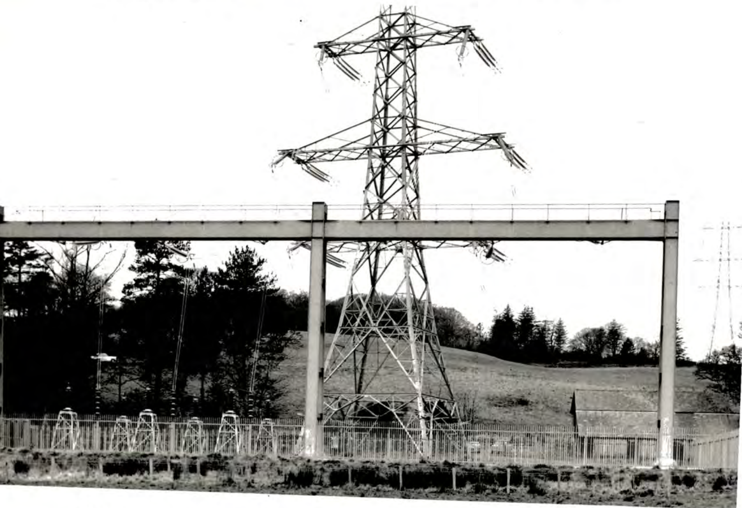
Photograph 30. Terminal tower and sealing end compound at Wern where 400 kV cable is connected to overhead line.
