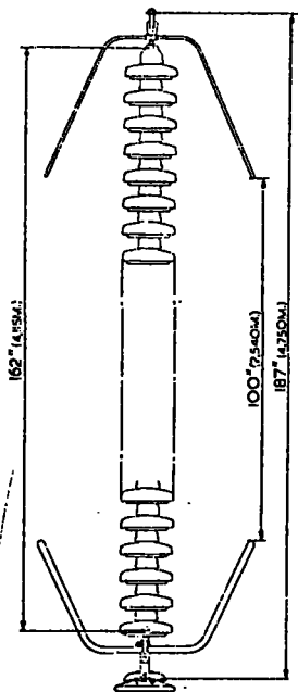
400 kV (twin)
