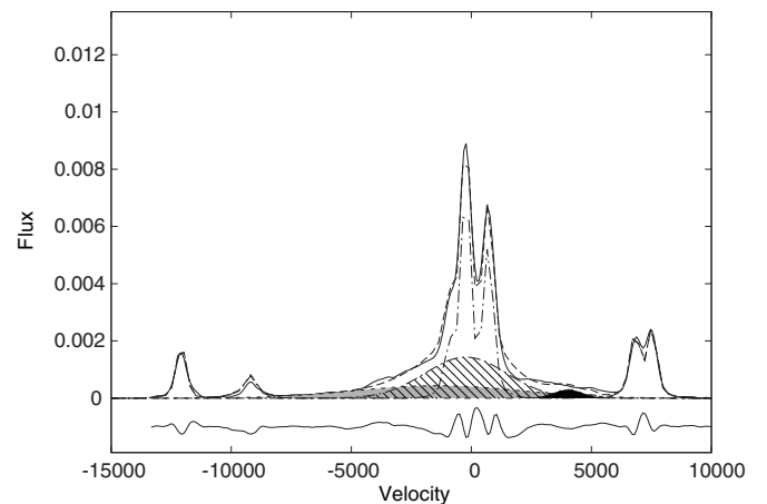
Figure 6. Same as in Figure 3, but for the spectrum obtained on Asiago 1.8 m Ekar telescope (epoch MJD 47609.529).
