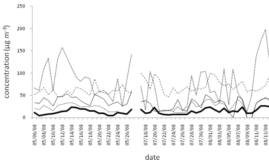
Figure 4. Correlations between concentrations of \text{PM}_{10} (—) determined in this work and concentrations of \text{NO}_x (---), \text{SO}_2 (—) and \text{*PM}_{10} (.....) obtained at automatic air-monitoring station during spring and summer campaigns at Omladinskih Brigada sampling site.
