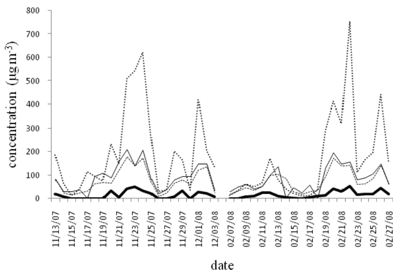
Figure 3. Correlations between concentrations of \text{PM}_{10} (—) determined in this work and concentrations of \text{NO}_x (---), \text{SO}_2 (—) and \text{*PM}_{10} (.....) obtained at automatic air-monitoring station during autumn and winter campaigns at Omladinskih Brigada sampling site.
