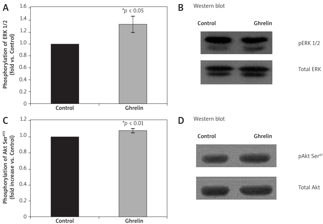
Figure 5. Effects of ghrelin on ERK1/2 (A and B) and Akt (C and D) phosphorylation in the rat liver. The results are expressed as a fold increase of control (CONTROL arbitrarily set at 1). Results are mean ± SEM of 4 separate experiments; p < 0.05 was considered significant (* p < 0.05 ; ** p < 0.01 ). B and D are representative Western blots ERK1/2 – phospho protein kinase p44/42, Akt – protein kinase B
