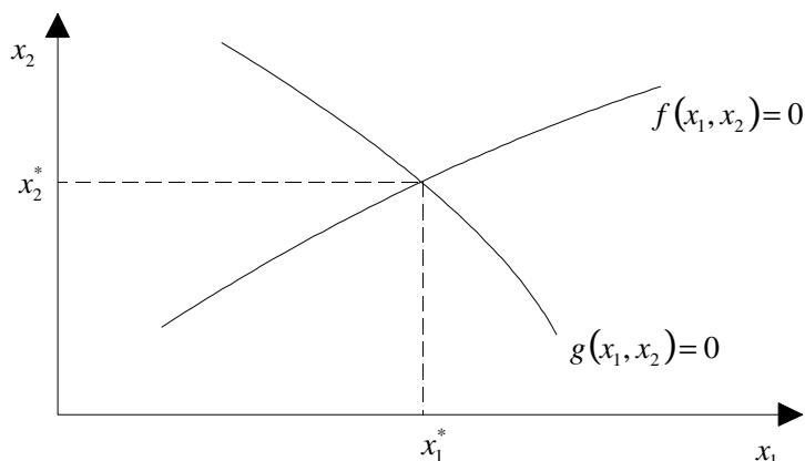
Figure 4.2.6 Zero motion lines with a unique steady state
