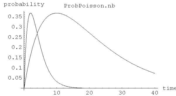
Figure 10.5.2 The probability of one jump by time \tau for a high arrival rate (peak at around 3) and a low arrival rate (peak at around 11)
