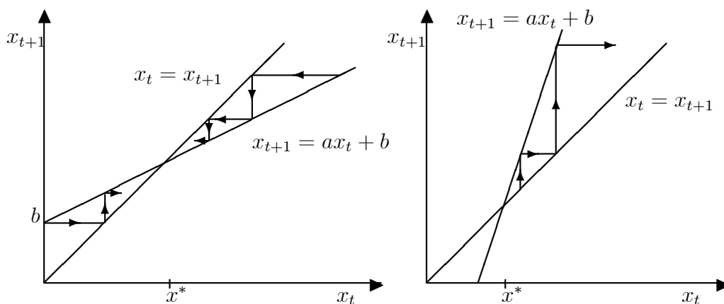
Figure 2.5.3 Phase diagrams of (2.5.6) for positive (left panel) and negative b (right panel) and higher a in the right panel
