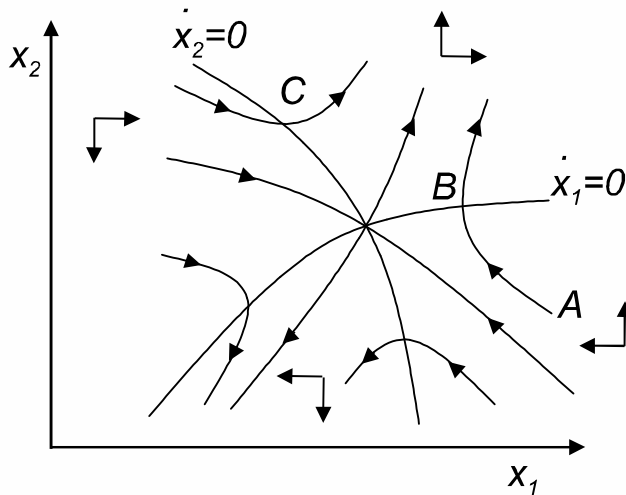
Figure 4.2.10 A saddle path
