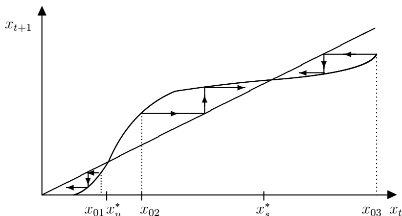
Figure 2.5.4 A locally stable fixpoint x_s^* and an unstable fixpoint x_u^*
