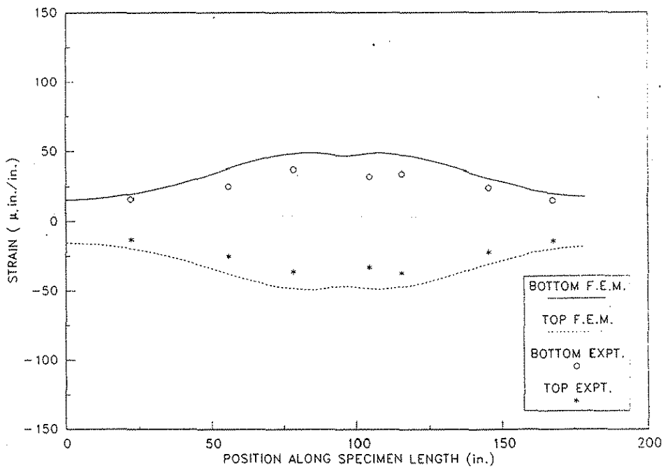
Figure 6.30. Midspan transverse strains along the specimen length for a double 20.8 kip load at Position Nos. 3C on Specimen No. 3.
