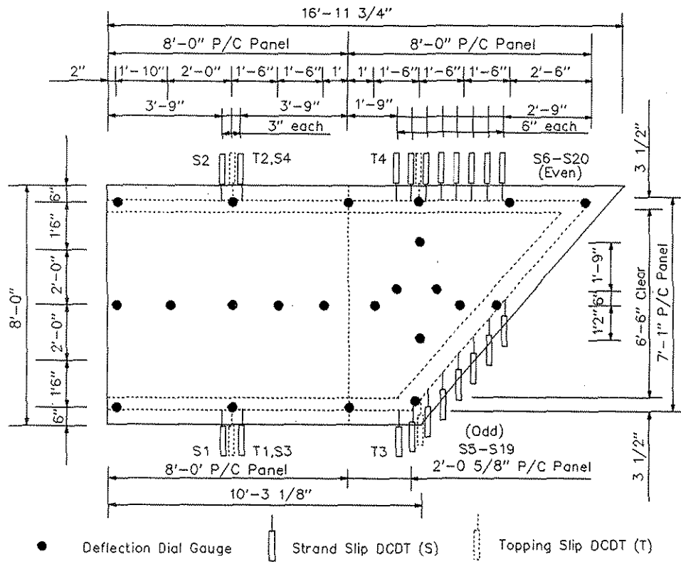
Figure 4.18. Dial gauge and DCDT locations for Specimen No. 5. (Load at Position No. 1D).
