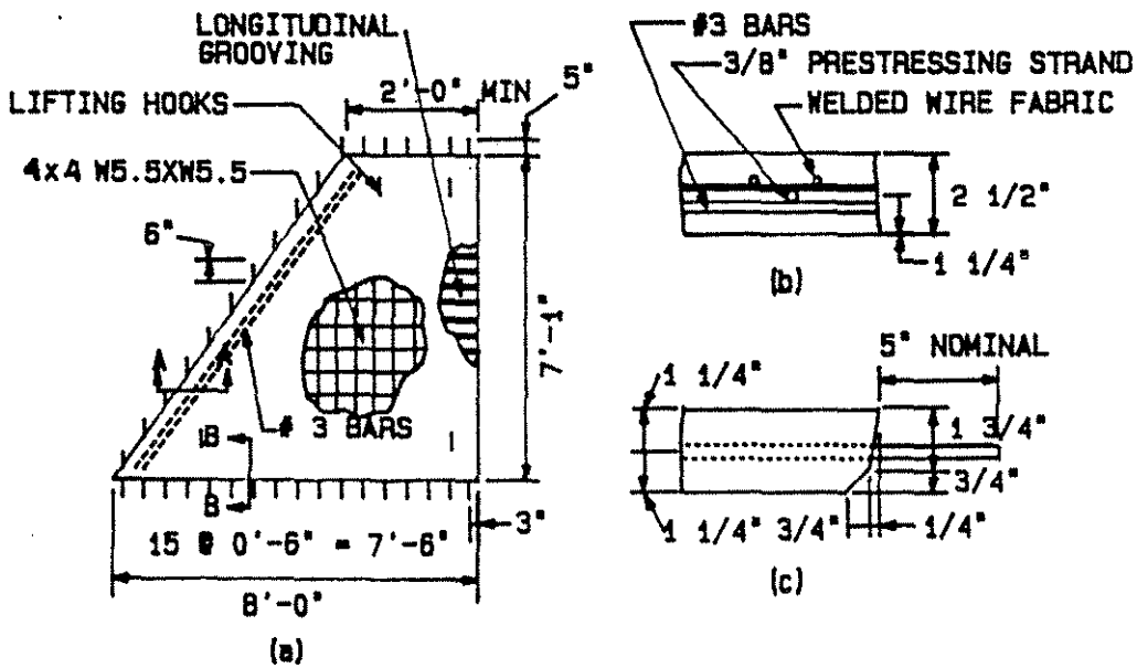
Figure 4.8. Trapezoidal precast prestressed concrete panel: (a) Plan view (b) Section A-A (c) Section B-B.
