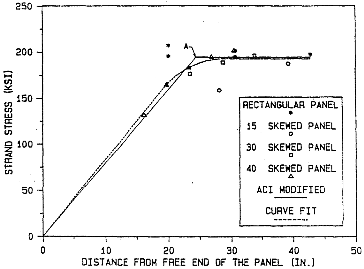
Figure 6.1. Strand embedment versus initial strand prestress.
