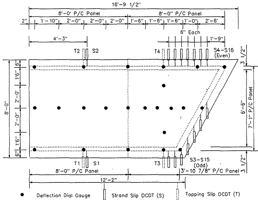
Figure 4.17. Dial gauge and DCDT locations for Specimen No. 4. (Load at Position No. 1C).
