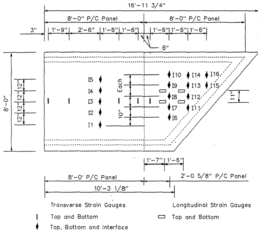
Figure 4.23. Strain gauge locations for Specimen No. 5.
