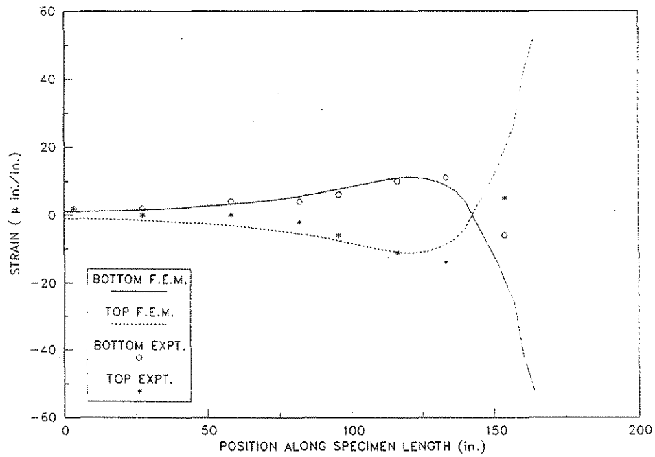
Figure 6.34. Midspan transverse strains along the specimen length for a single 48 kip load at Position No. 2E on Specimen No. 4.
