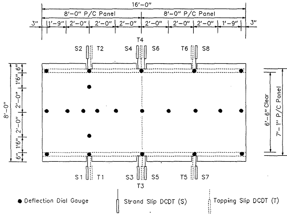
Figure 4.14. Dial gauge and DCDT locations for Specimen No. 1. (Load at Position No. 1A).
