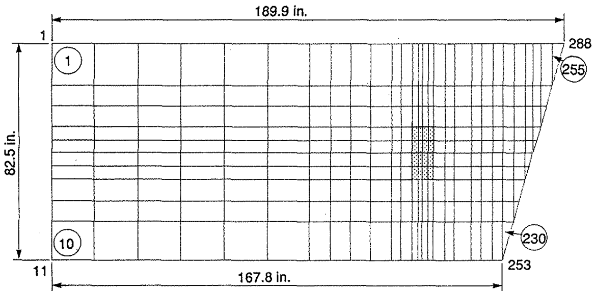
Figure 5.4. Finite element model for wheel load at Position No. 1E on Specimen No. 3.
