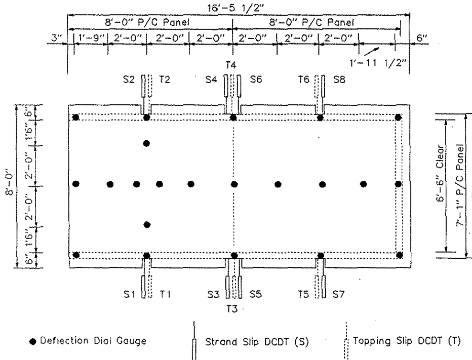
Figure 4.15. Dial gauge and DCDT locations for Specimen No. 2. (Load at Position No. 1A).
