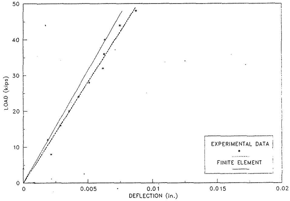
Figure 6.18. Load versus deflection for a single load at Position No. 1D on Specimen No. 4.
