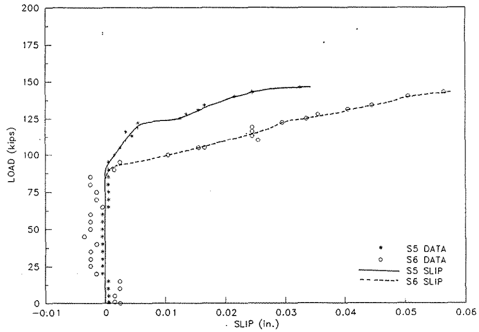
Figure 6.2. Strand-slip at S5 and S6 during ultimate load test on Specimen No. 1.
