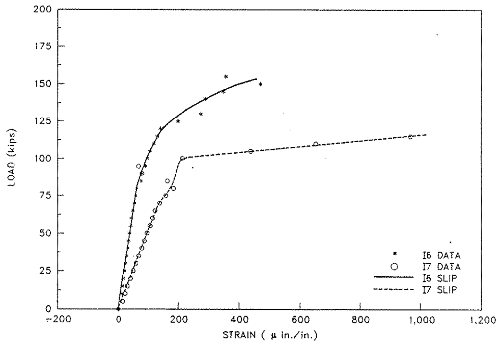
Figure 6.9. Interface-slip at I6 and I7 during Ultimate Strength Test No. 1 on Specimen No. 5.
