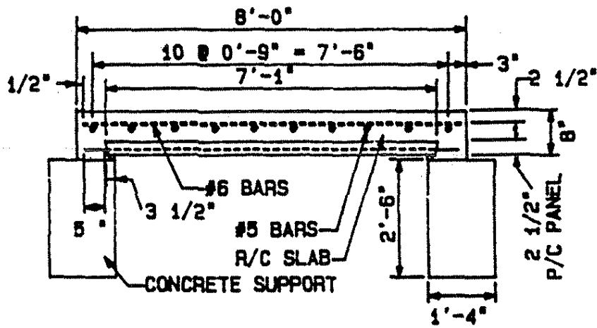
Figure 4.6 Cross section of composite specimen.
