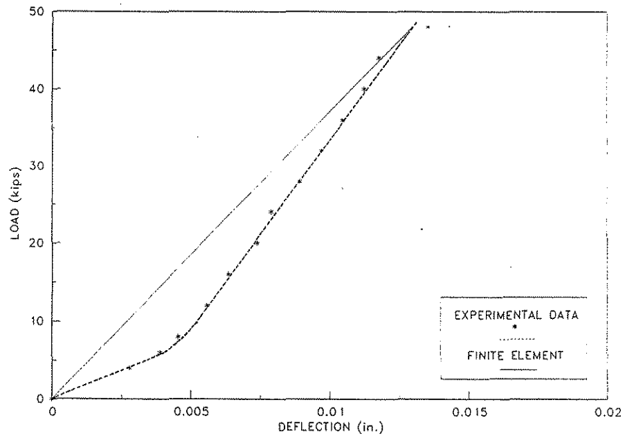
Figure 6.20. Load versus deflection for a single load at Position No. 1D on Specimen No. 5.
