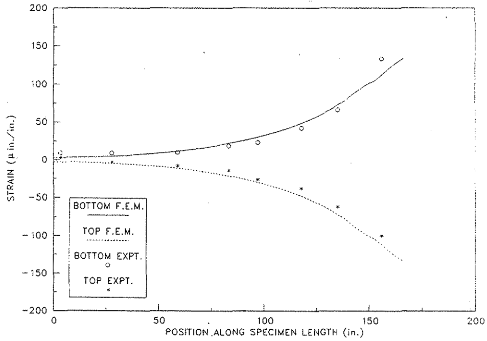
Figure 6.33. Midspan transverse strains along the specimen length for a single 48 kip load at Position No. 1D on Specimen No. 4.
