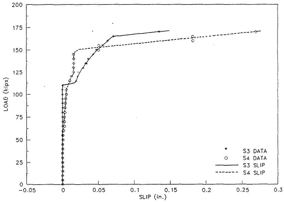
Figure 6.4. Strand-slip at S3 and S4 during Ultimate Test No. 1 on Specimen No. 4.
