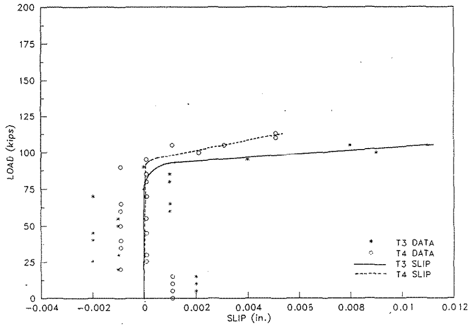
Figure 6.10. Topping-slip at T3 and T4 during Ultimate Load Test on Specimen No. 1.
