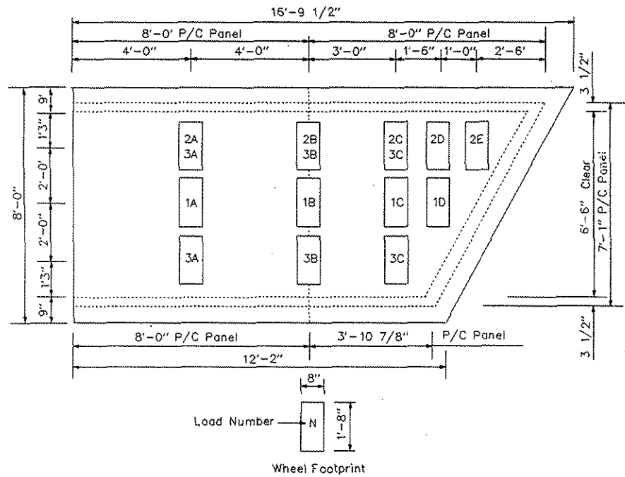
Figure 4.12. Load positions for Specimen No. 4.
