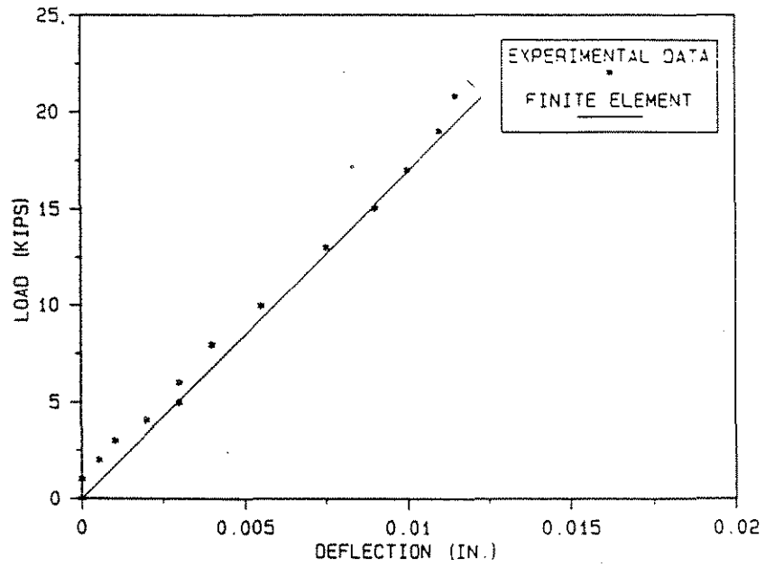
Figure 6.14. Load versus deflection for a single load at position No. 1A on Specimen No. 1.
