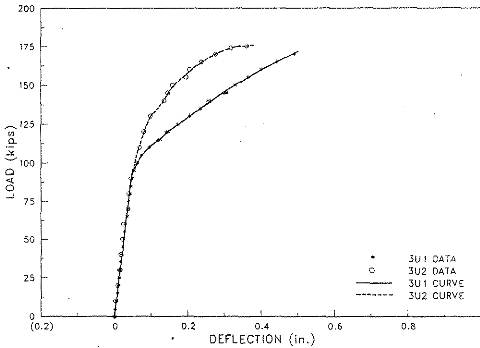
Figure 6.24. Load versus deflection for the Ultimate Load Tests on Specimen No. 3 (Load at Position Nos. 1E for 3U1 and 1.5 ft. above 1A for 3U2).
