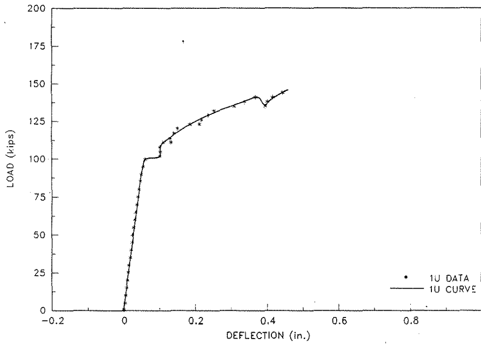
Figure 6.22. Load versus deflection for the Ultimate Lead Test on Specimen No. 1 (Load at Position No. 1C).
