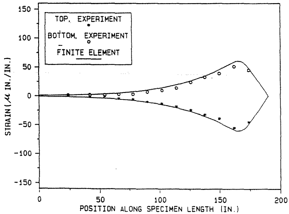
Figure 6.28. Midspan transverse strains along the specimen length for a single 20.8 kip load at Position No. 1E on Specimen No. 2.
