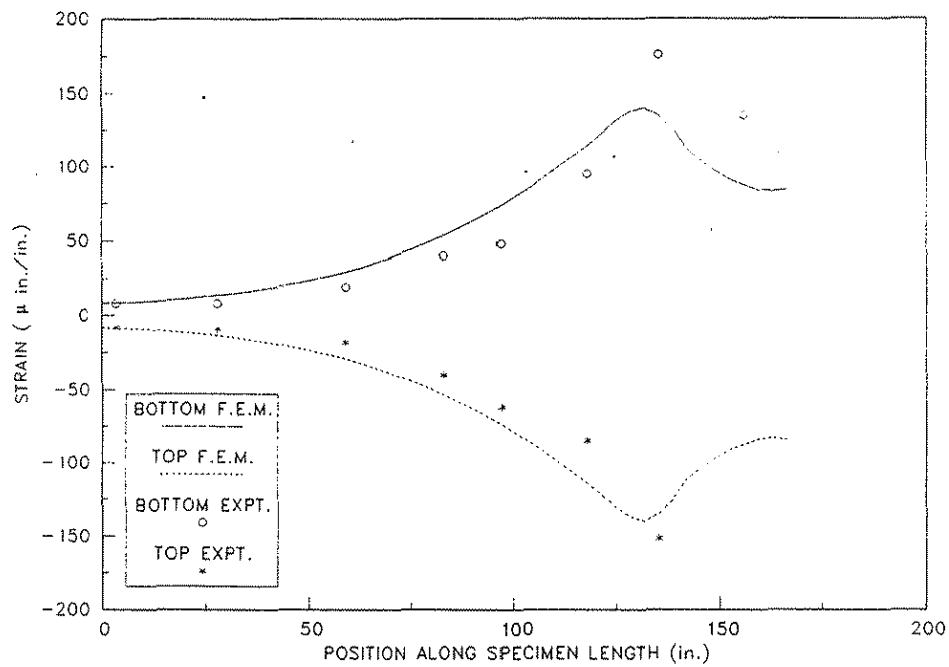
Figure 6.32. Midspan transverse strains along the specimen length for a single 48 kip load at Position No. 1C on Specimen No. 4.
