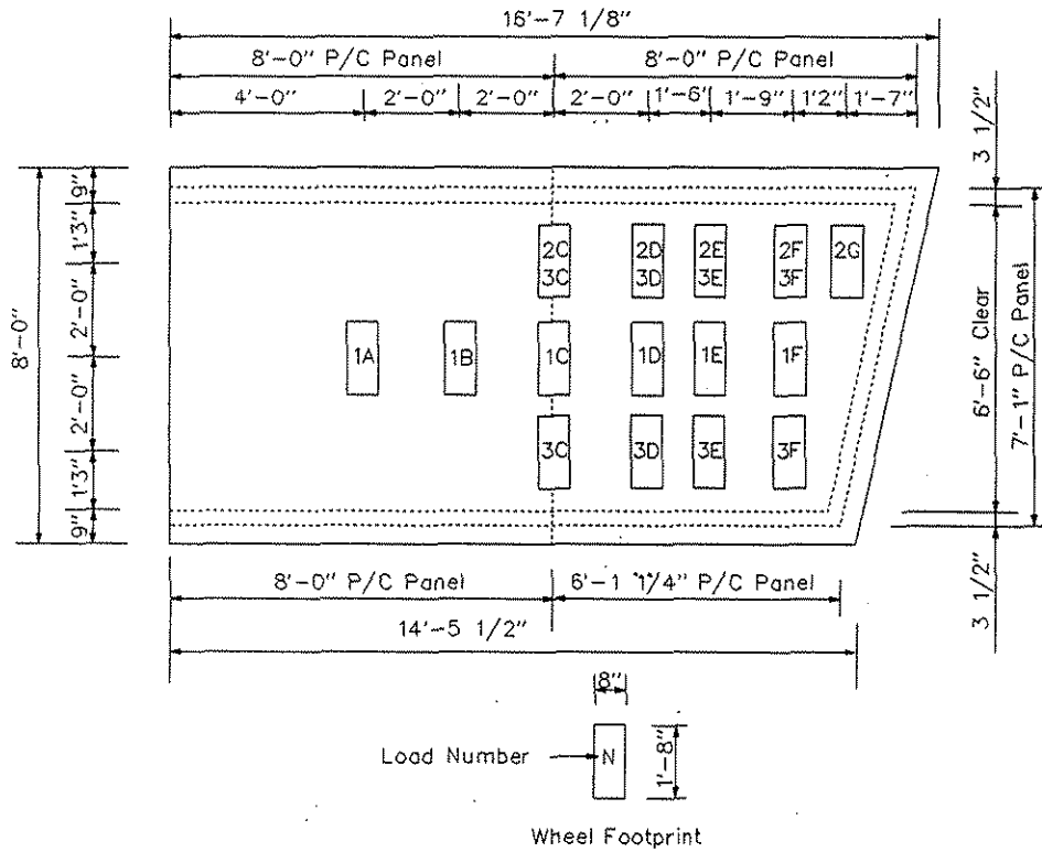
Figure 4.11. Load positions for Specimen No. 3.
