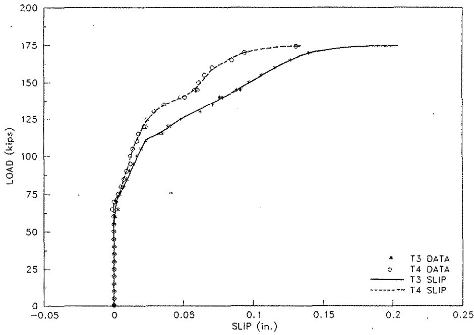
Figure 6.13. Topping-slip at T3 and T4 during Ultimate Test No. 1 on Specimen No. 5.
