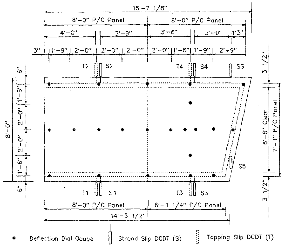
Figure 4.16. Dial gauge and DCDT locations for Specimen No. 3. (Load at Position No. 1E).
