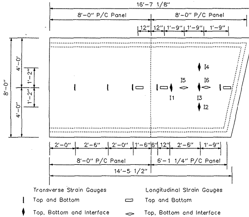
Figure 4.21. Strain gauge locations for Specimen No. 3.
