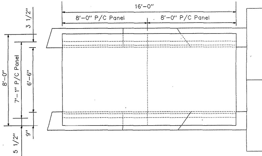
Figure 4.1. Specimen No. 1 configuration.
