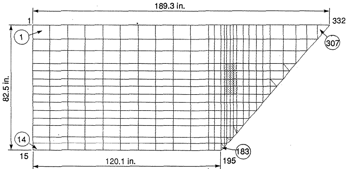
Figure 5.6. Finite element model for wheel load at Position 1D on Specimen No. 5.
