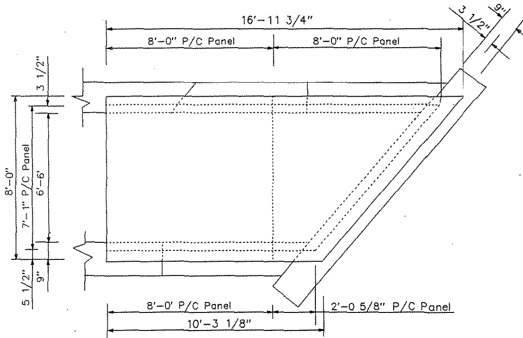
Figure 4.5. Specimen No. 5 configuration.
