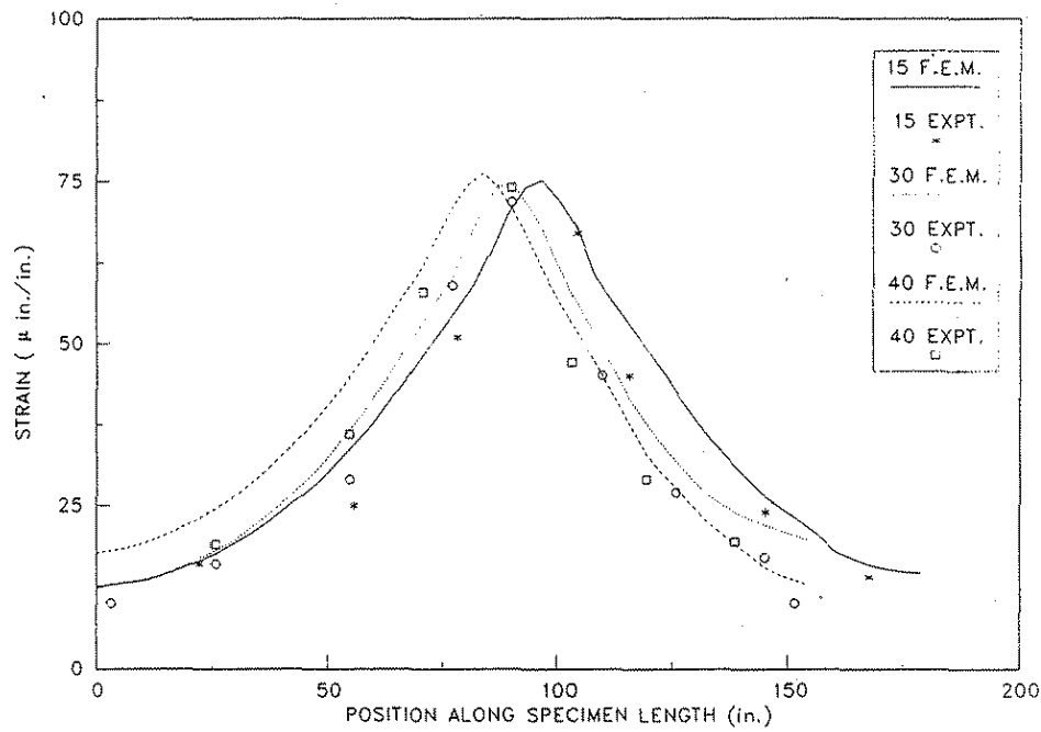
Figure 6.29. Bottom midspan transverse strains along the specimen length for a single 20.8 kip load applied near or above the panel joint on Specimen No. 3, 4, and 5.
