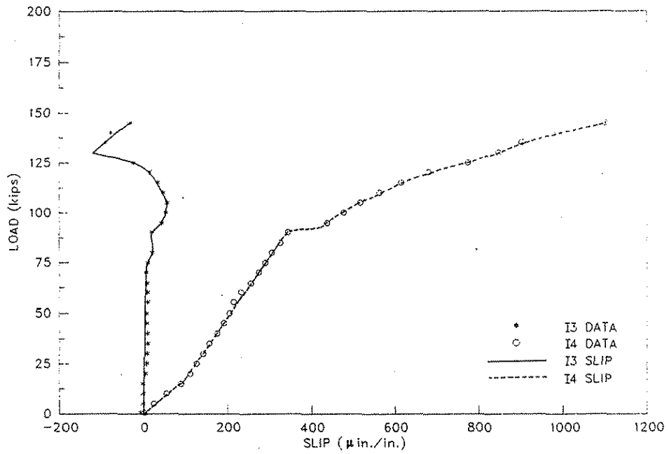
Figure 6.7. Interface - slip at I3 and I4 during Ultimate Load Test No. 1 on Specimen No. 2.
