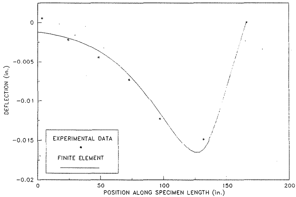
Figure 6.21. Midspan deflection along the specimen length for a single 48 kip load at Position No. 1C on Specimen No. 4.
