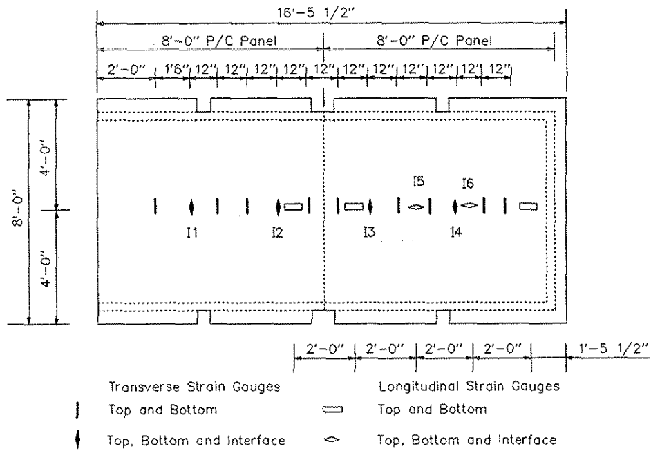
Figure 4.20. Strain gauge locations for Specimen No. 2.
