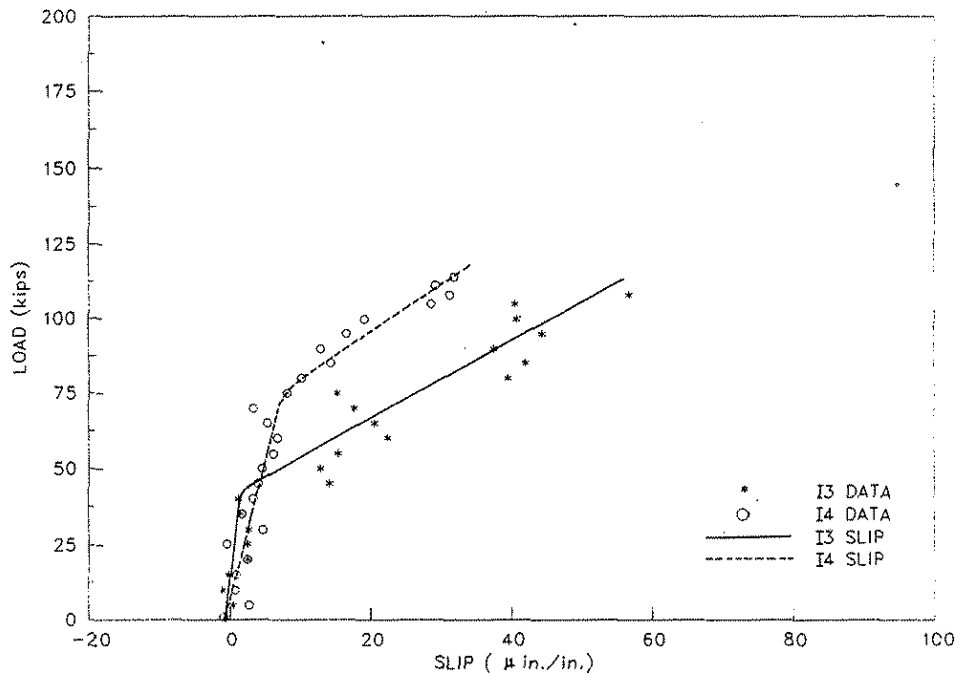
Figure 6.6. Interface-slip at I3 and I4 during Ultimate Test No. 1 on Specimen No. 1.
