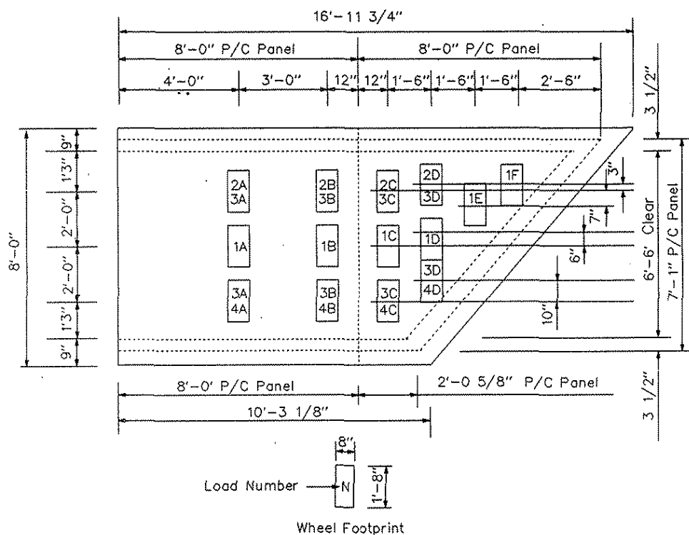
Figure 4.13. Load position for Specimen No. 5.
