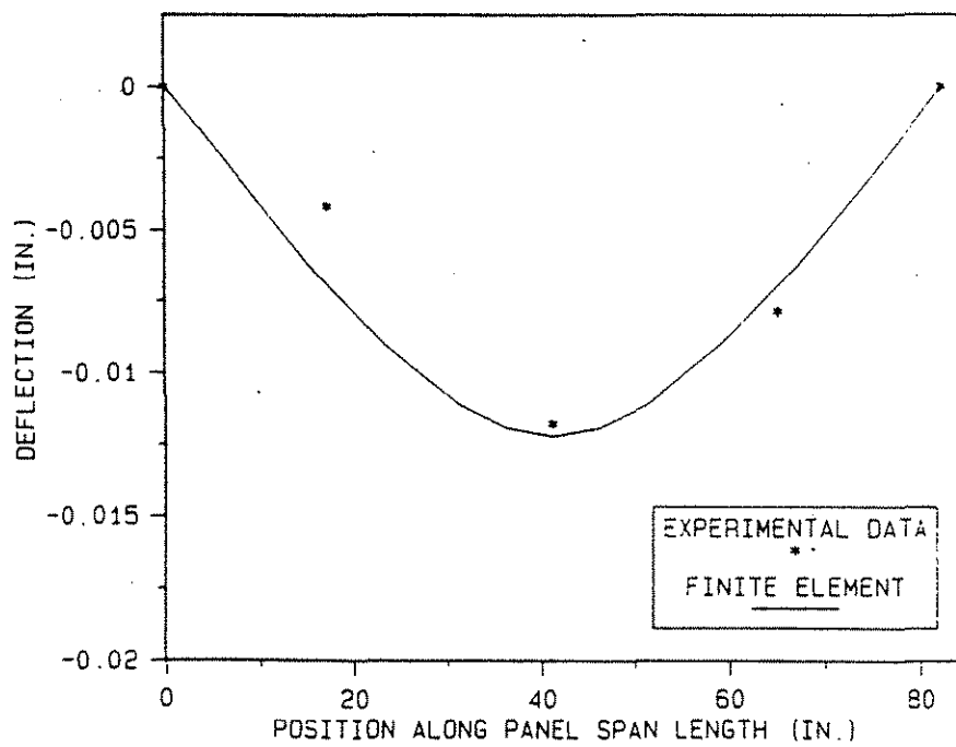
Figure 6.15. Deflections along the precast panel span for a single 20.8 kip load at No. 1A on Specimen No. 1.
