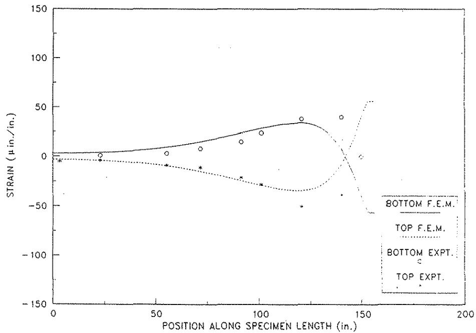
Figure 6.36. Midspan transverse strains along the specimen length for a single 48 kip load at Position No. 1E on Specimen No. 5.
