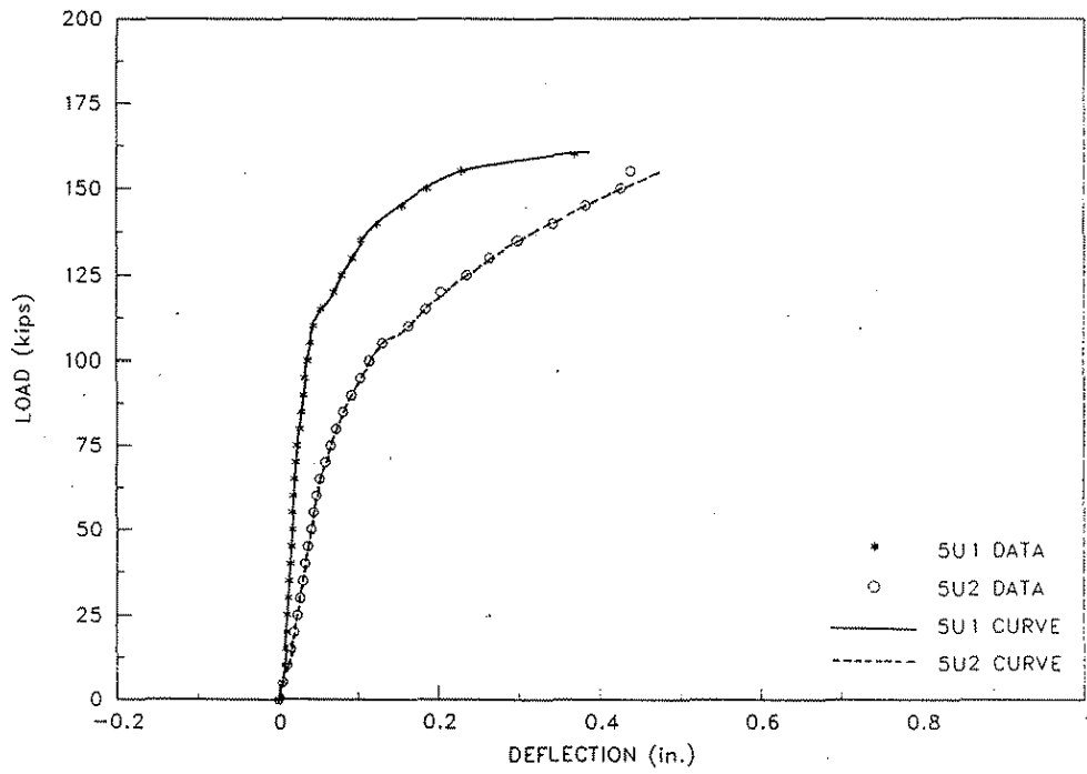
Figure 6.26. Load versus deflection for the Ultimate Load Tests on Specimen No. 5 (Load at Position Nos. 1D for 5U1 and 1.3 ft. above 1A for 5U2).
