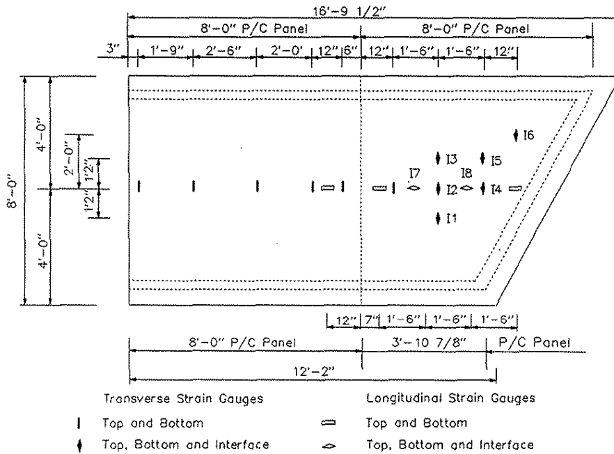
Figure 4.22. Strain gauge locations for Specimen No. 4.
