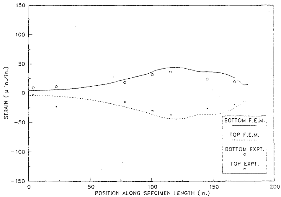
Figure 6.31. Midspan transverse strains along the specimen length for a double 20.8 kip load at Position Nos. 3E on Specimen No. 3.
