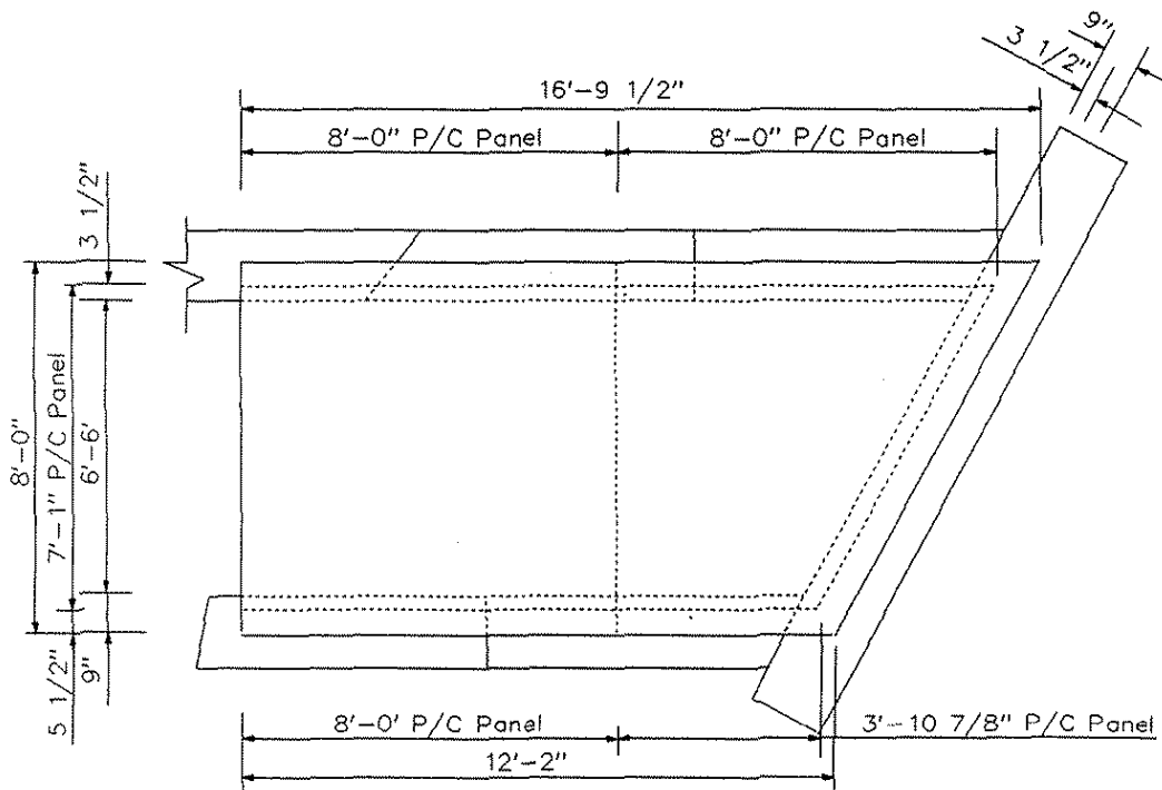
Figure 4.4. Specimen No. 4 configuration.
