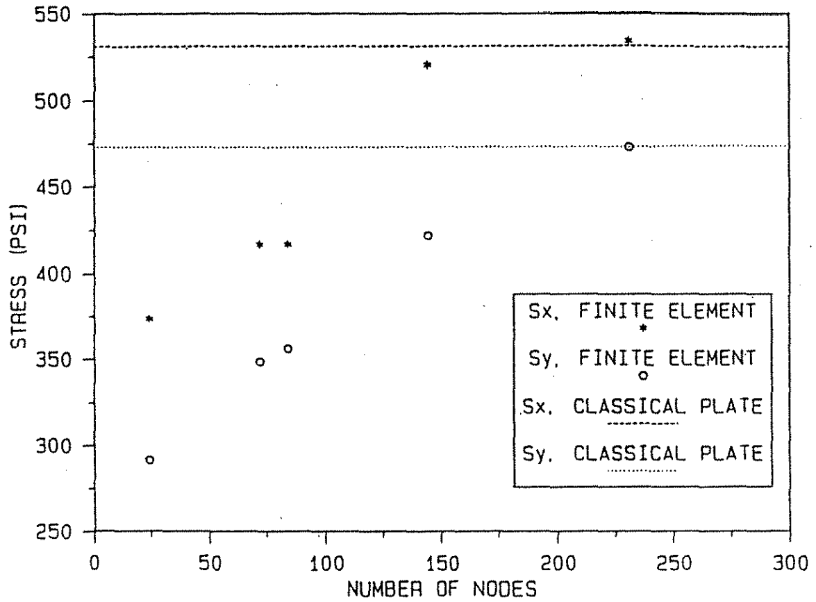
Figure 5.2. Mesh size effects on slab stresses.
