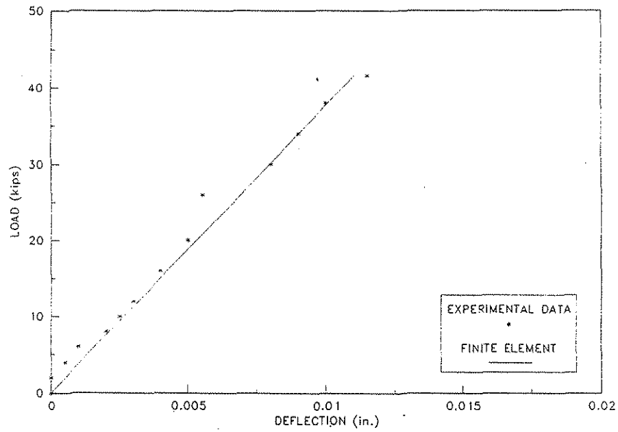
Figure 6.16. Load versus deflection for a double load at Position Nos. 3C on Specimen No. 3.
