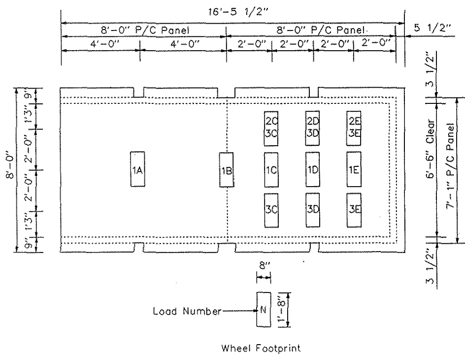
Figure 4.10. Load positions for Specimen No. 2.
