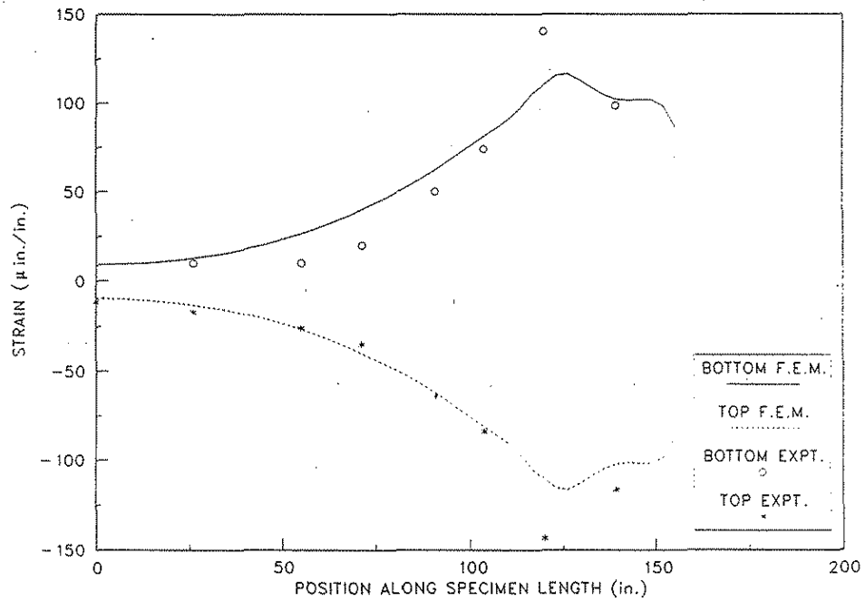
Figure 6.35. Midspan transverse strains along the specimen length for a single 48 kip load at Position No. 1D on Specimen No. 5.
