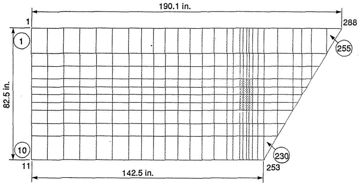
Figure 5.5. Finite element model for wheel load at Position 1C on Specimen No. 4.
