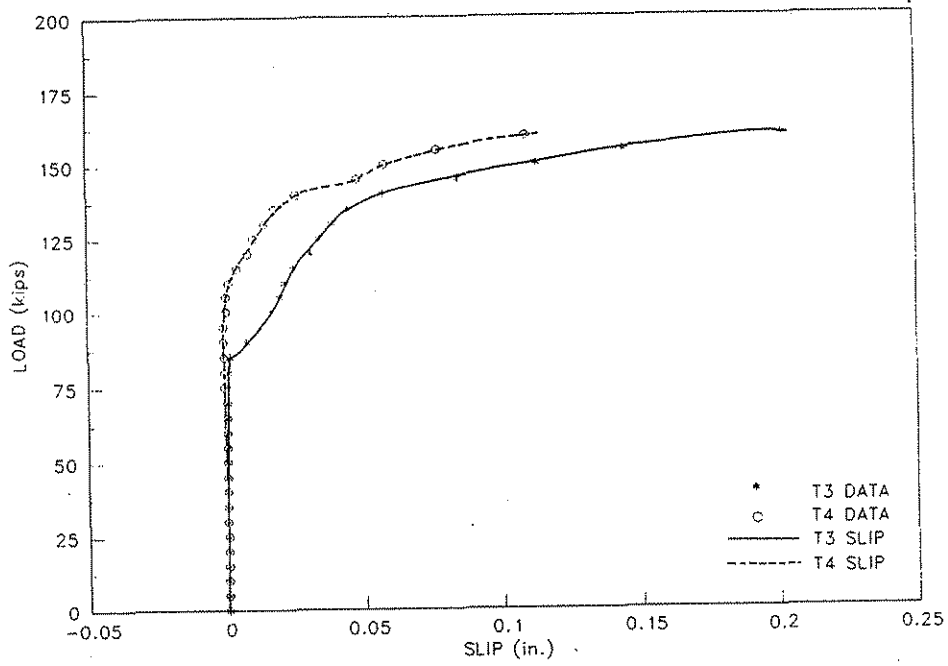
Figure 6.12. Topping-slip at T3 and T4 during Ultimate Test No. 1 on Specimen No. 3
