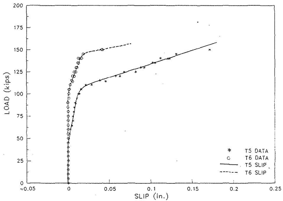
Figure 6.11. Topping-slip at T5 and T6 during Ultimate Strength Test No. 1 on Specimen No. 2.
