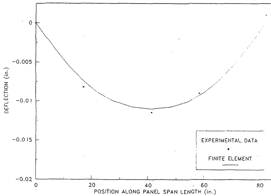
Figure 6.17. Deflections along the precast panel span for a double 20.8 kip load at Position Nos. 3C on Specimen No. 3.
