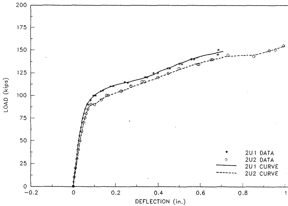
Figure 6.23. Load versus deflection for the Ultimate Load Tests on Specimen No. 2 (Load at Position Nos. 1D for 2U1 and at 1A for 2U2).
