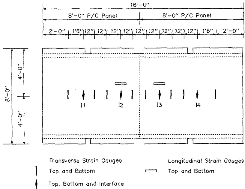
Figure 4.19. Strain gauge locations for Specimen No. 1.
