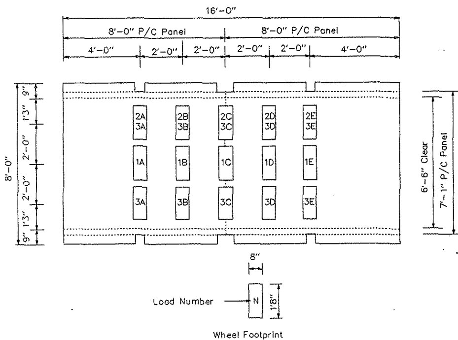
Figure 4.9. Load positions for Specimen No. 1.
