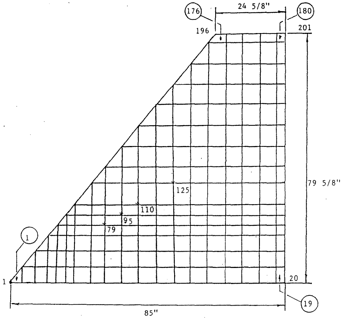
Figure 5.1. Finite element panel model for the 40 degree skewed configuration.
