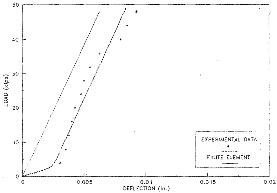
Figure 6.19. Load versus deflection for a single load at Position No. 2E on Specimen No. 4.
