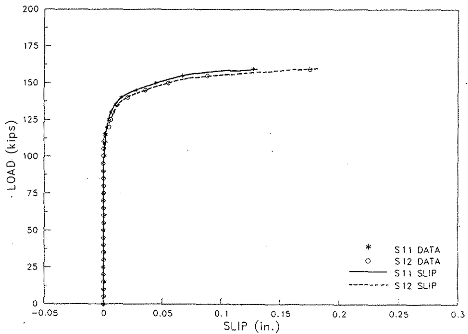
Figure 6.5. Strand-slip at S11 and S12 during Ultimate Test No. 1 on Specimen No. 5.
