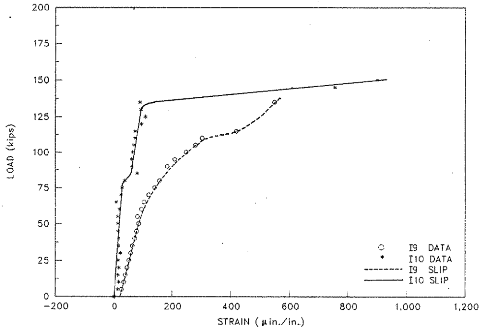
Figure 6.8. Interface-slip at I9 and I10 during Ultimate Test No. 1 on Specimen No. 5.
