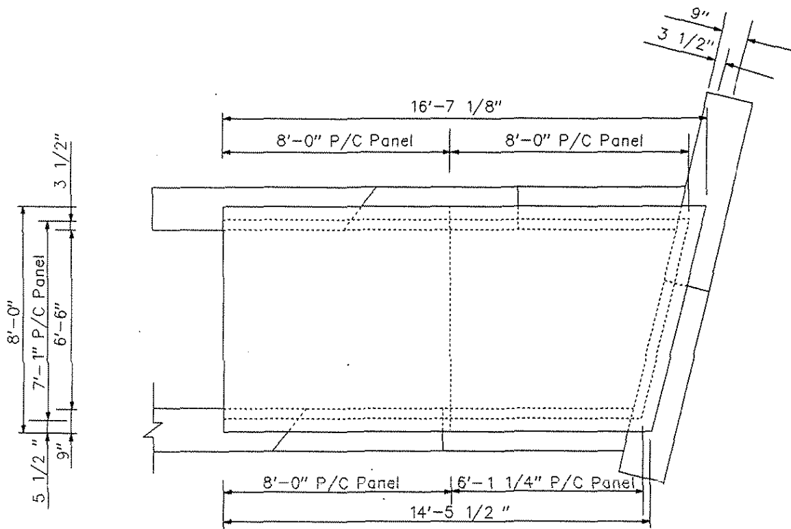
Figure 4.3. Specimen No. 3 configuration.
