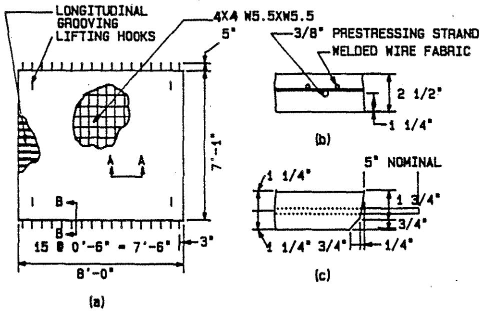
Figure 4.7. Rectangular precast prestressed concrete panel: (a) Plan view (b) Section A-A (c) Section B-B.
