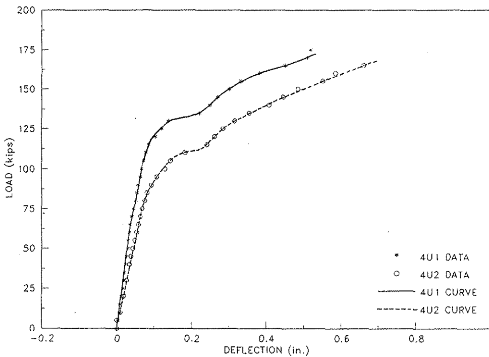
Figure 6.25. Load versus deflection for the Ultimate Load Tests on Specimen No.4 (Load at Position Nos. 1C for 4U1 and at 1A for 4U2).
