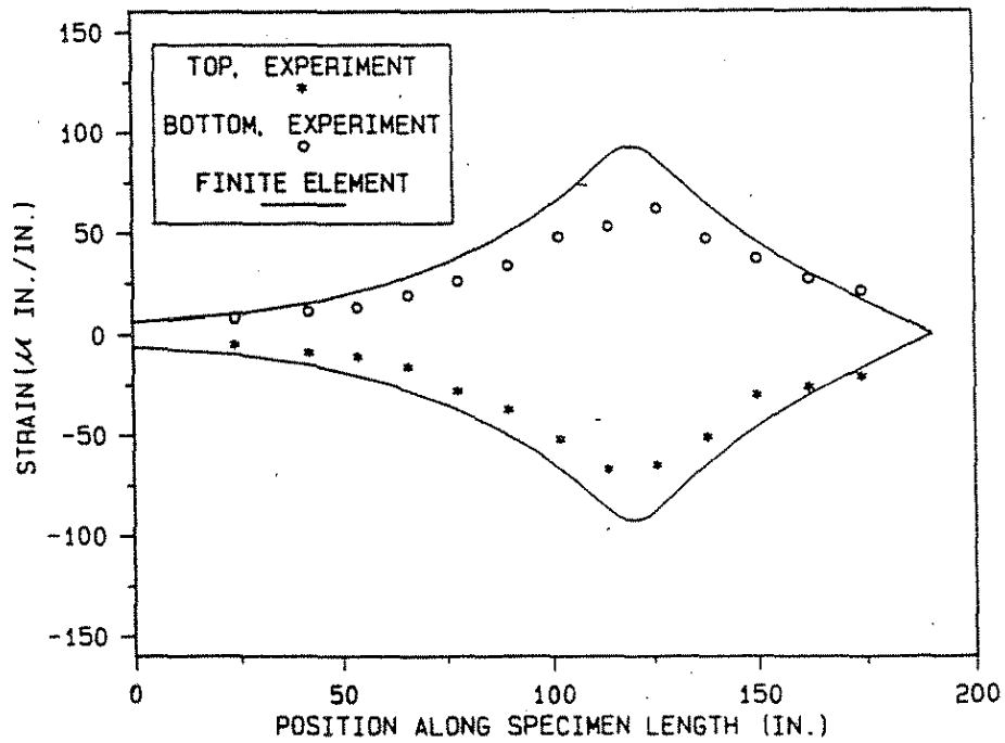
Figure 6.27. Midspan transverse strains along the specimen length for a single 20.8 kip load at Position No. 1C on Specimen No. 2.
