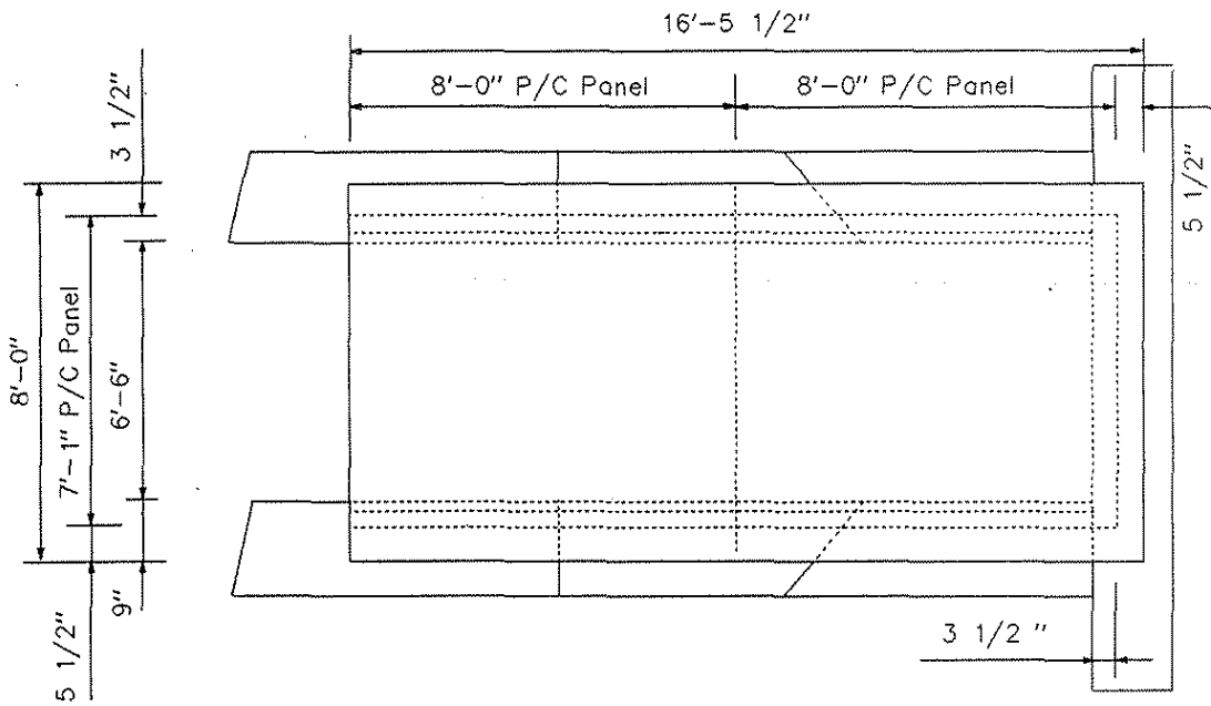
Figure 4.2. Specimen No. 2 configuration.
