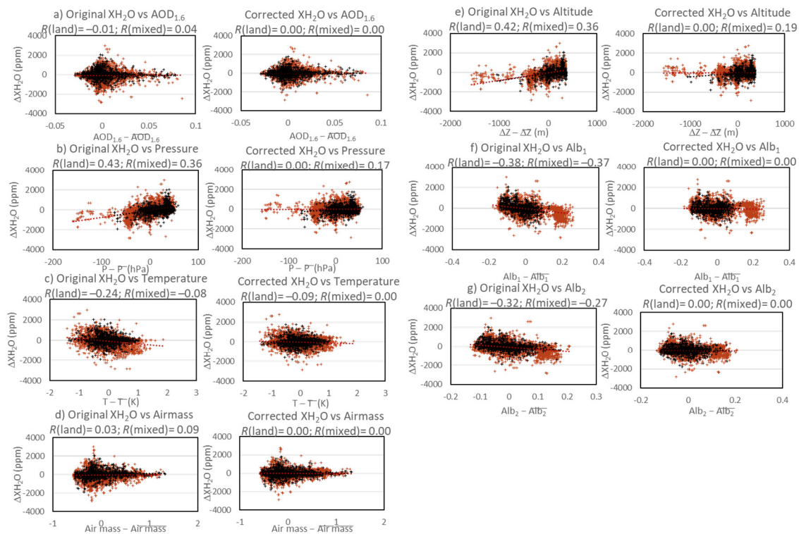
Figure 3. Scatter plots between \Delta XH_2O calculated from original GOSAT SWIR XH 2 O data (left panels) or from GOSAT SWIR XH 2 O data corrected by bias-correction method (E) (right panels) and auxiliary parameters (a) AOD 1.6 , (b) surface pressure, (c) temperature shift, (d) air mass, (e) altitude, (f) Alb 1 , and (g) Alb 2 for case 1. Red symbols indicate GOSAT gain H land data, and black symbols indicate GOSAT gain H mixed for case 1. Red symbols indicate GOSAT gain H land data and black symbols
