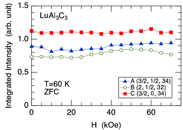
Fig. 9. (Color online) Magnetic field dependences of the superlattice peak intensities corresponding to the three orthorhombic domains of \text{LuAl}_3\text{C}_3 at \psi = 0^\circ .
