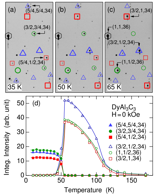
Fig. 4. (Color online) (a)(b)(c) Selected area of oscillation photographs of \text{DyAl}_3\text{C}_3 , demonstrating the disappearance and appearance of the superlattice peaks shown in Figs. 1(b) and 1(c) when crossing the phase boundary at 50 K. Small thin marks and large thick marks are peaks appearing below and above 50 K, respectively. Hexagons, triangles, circles, and squares represent Bragg spots of fundamental lattice, domain A, domain B, and domain C, respectively. (d) Temperature dependences of the peak intensities, which are indexed in (a) and (c).
