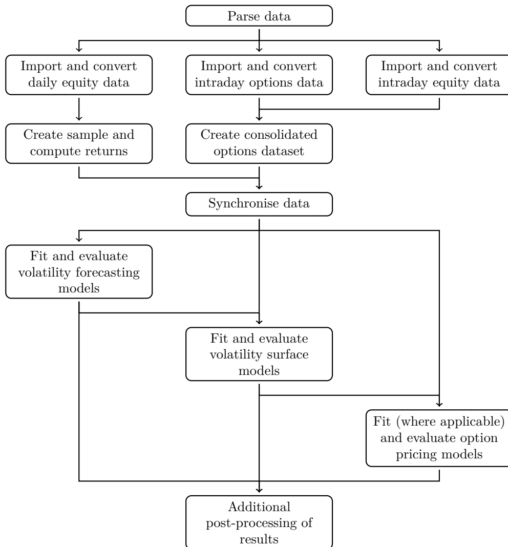
Figure 3.7: Schematic Overview of the Model Development and Processing Workflow
