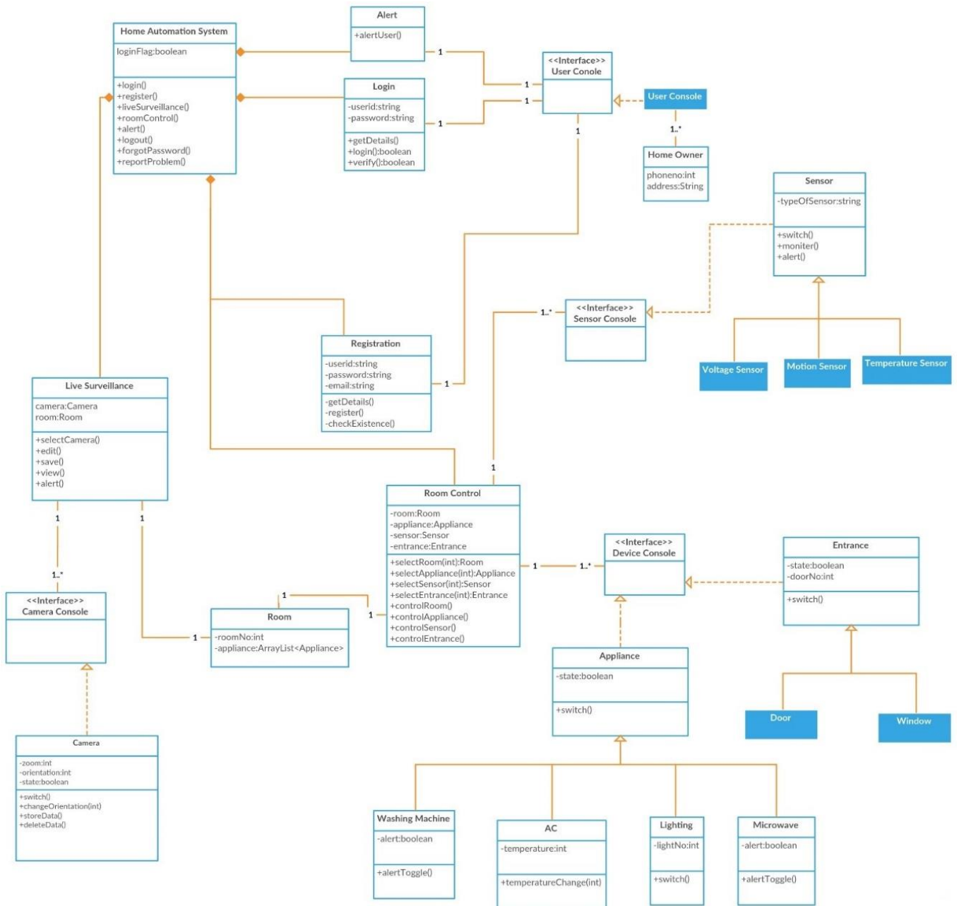
Figure 11: Class Diagram of Smart Home Automation
