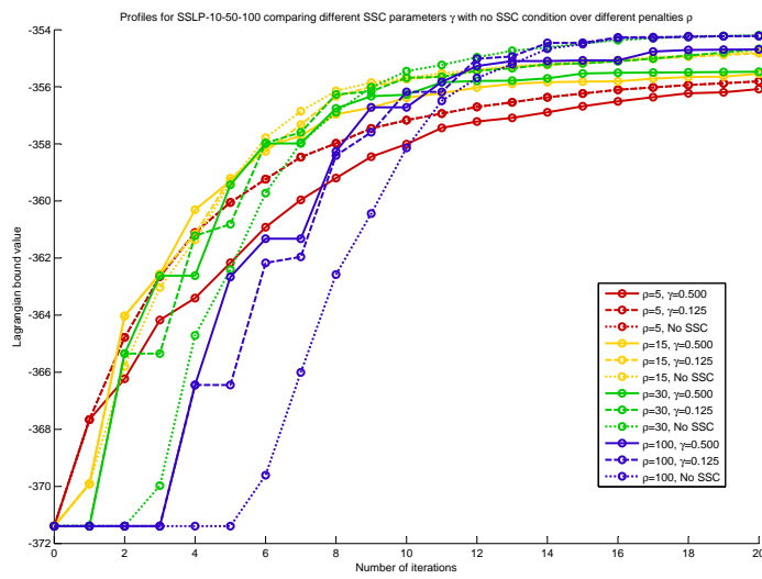
Fig. 4 Applying SDM-GS-ALM to SSLP-10-50-100 using different parameterizations for the SSC condition (or none).
