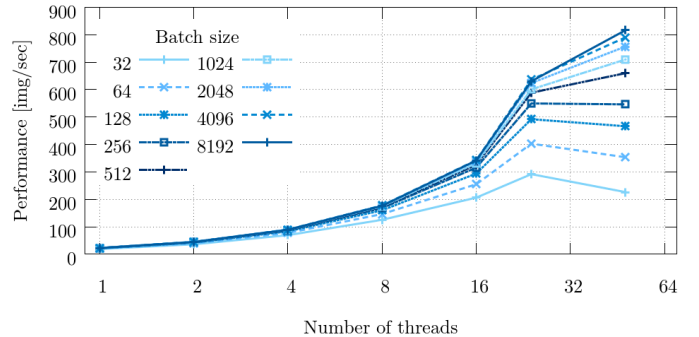
Fig. 3. Thread Scaling of AlexNet with MKL version on one node of MareNostrum4
