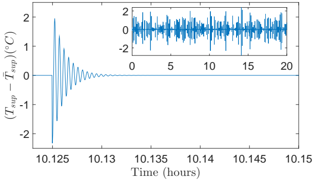
Fig. 4. Plot of the response of (T_{sup} - \bar{T}_{sup}) during the simulation for 4 selected racks. The full simulation is shown in the inset and the main plot is a magnification of the response after a change in total workload around t = 10 hours. The controller successfully drives the system to the new optimal value under varying total workload. The initial overshoot depends on the change of the total workload, i.e. the difference between the optimal supply temperatures in the two intervals. The oscillatory response results in an oscillatory fluctuation in the output temperature profile.
