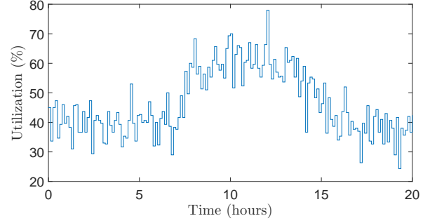
Fig. 2. Synthetic workload trace supplied to data center. The workload varies \pm 10\% about two nominal values, representing nighttime and daytime operation levels. The total workload changes every 7.5 minutes during which the workload is assumed to be constant.
