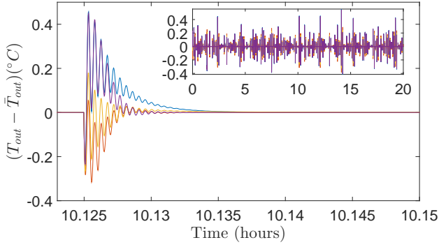
Fig. 3. Plot of the response of (T_{out} - \bar{T}_{out}) during the simulation for 4 selected racks. The full simulation is shown in the inset and the main plot is a magnification of the response after a change in total workload around t = 10 hours. Each time the total workload changes, the temperature of the racks start to deviate from the optimal value and the controllers drive the data center to the new optimal solution, (T_{out} - \bar{T}_{out}) = 0 again. The oscillatory response of the output temperature coincides with the response of the supply temperature controller. Over the whole simulation the temperature is kept in a bandwidth of \pm 0.5 °C around the target temperature distribution.
