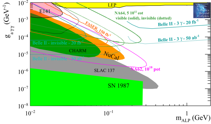
Figure 37: BC9: ALPs with photon coupling. Current bounds (filled areas) and prospects for PBC projects on 5 years timescale (solid lines) in the plane coupling g_{a\gamma\gamma} versus mass m_{ALP} . The results from a phenomenological study for Belle-II [303] is also shown.
